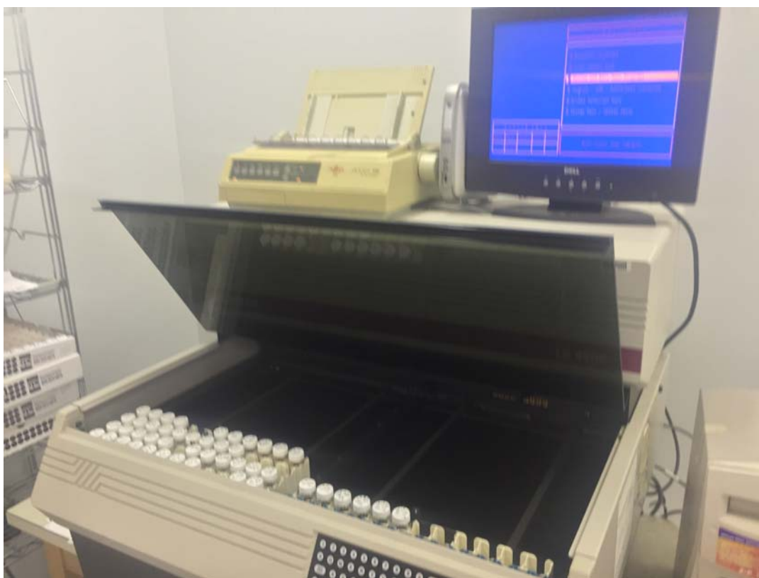
Figure 1. The Beckman LS 6500 Scintillation System used at Sagamore Adams Laboratories in Lafayette, Indiana.
