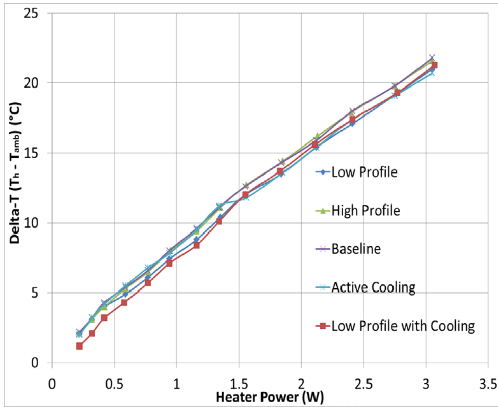
Figure 8. Plot of Change in Heater Temperature at 0° Orientation
