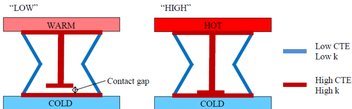
Figure 2. A thermal switch concept based on the deformation of C3M device
