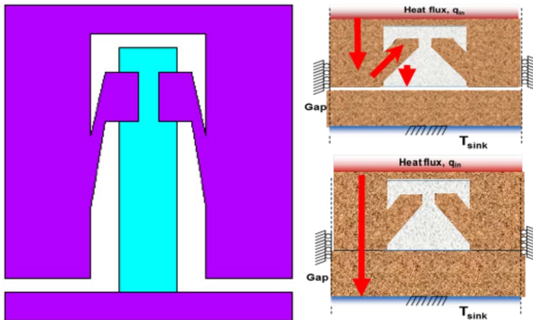
Figure 8. (left) design from (Staveland 2013); (right) fabricated thermal switch, 'open' and 'closed'
