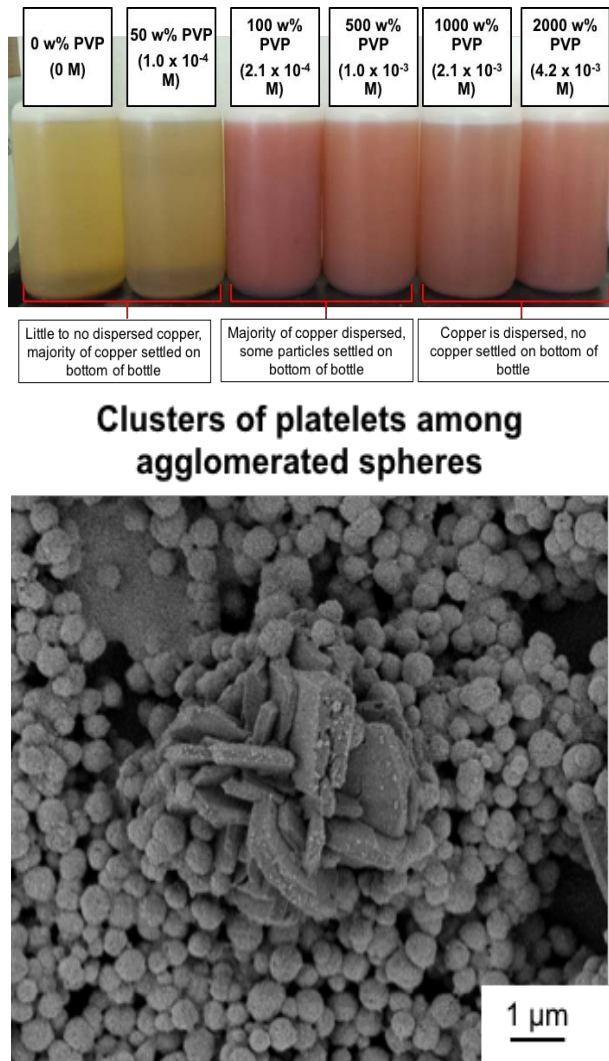
Figure 4. (top) Copper nanoparticle dispersion and (bottom) photomicrograph of 500 w/o PVP sample
