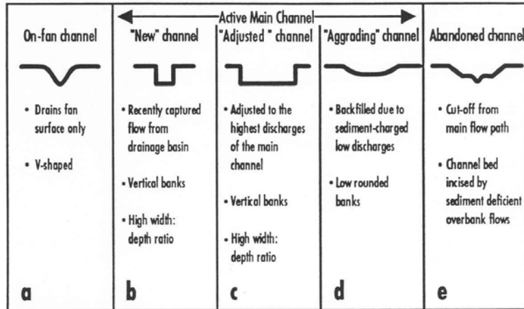
Figure 38. An example of classifications for arid-region rivers: channel morphologies characteristic of alluvial fans in the southwestern United States. Morphologic types can change with time and space (from Field 2001 and Field and Lichvar 2007, Fig. 9).
