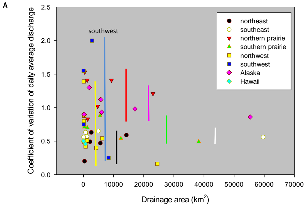
Figure 71. Graphical illustration of regional differences in coefficient of variation (CV) for (A) average daily discharge and (B) peak annual discharge. The colored vertical bars represent the range of CV values for each region. Rivers of the southwestern United States have by far the largest range and the greatest values whereas rivers of the northeastern and southeastern regions have low average values and a relatively small range within each region. The highest value for the southwest in (B) extends well beyond the maximum value on the y-axis; the highest value was not included to make it easier to discern relative variations among the other regions.
