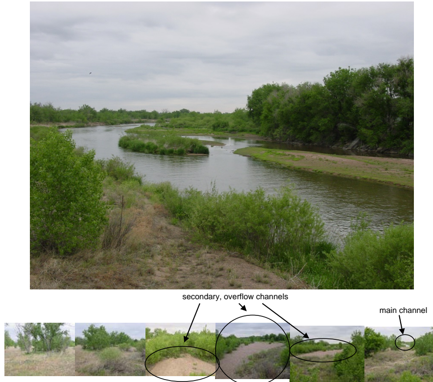
Figure 60. Examples of shortgrass prairie channels. The South Platte River in eastern Colorado is now a single channel lined by riparian woodlands. Prior to flow regulation, the channel was braided and had minimal woody vegetation. The lower photo mosaic illustrates the extent of the former active channel when the river was braided.
