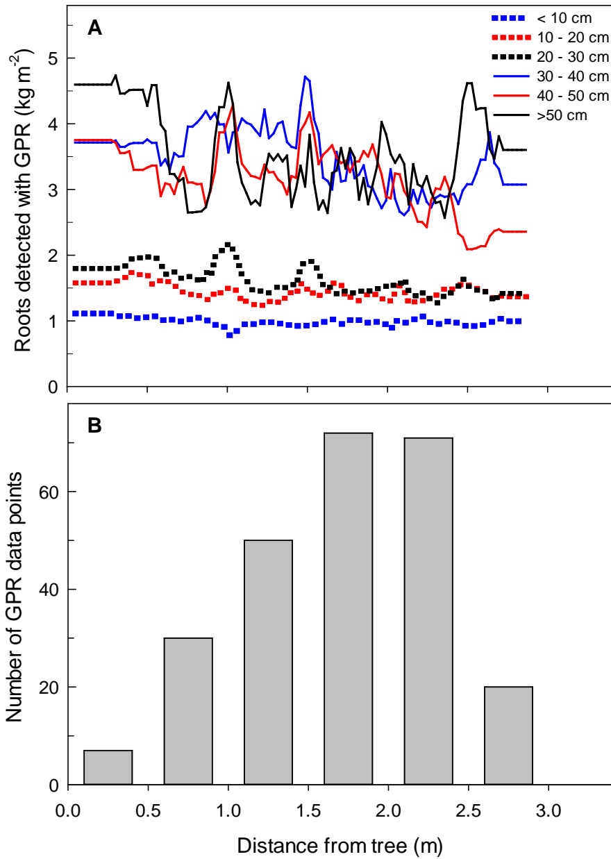
Figure 6.6. Root mass detected with GPR in the entire 16 \text{ m}^2 sample area plotted as distance from tree (A). Data were averaged by DBH class (<10, 10-20, 20-30, 30-40, 40-50, >50 cm) resulting in 252 mass/distance observations per class. The data were smoothed using a running average filter with a sampling proportion of 0.05. The distribution of GPR data points as related to distance from tree are presented in inset B.
