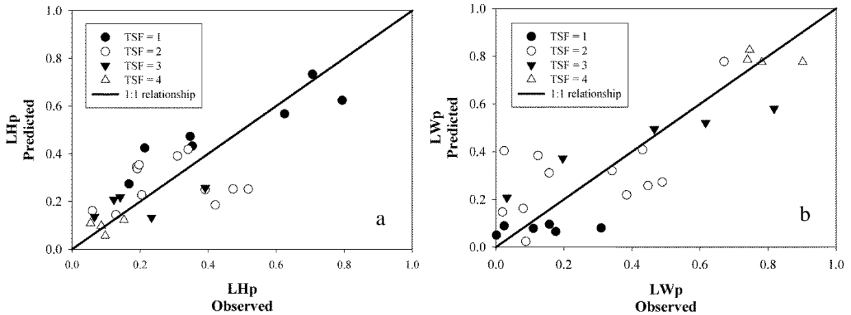
Figure 13.5. Relationship between observed and predicted a) ratio of living herbaceous (LHp) and b) ratio of living woody (LWp) to total ground cover biomass for different time since last prescribed fire (TSF) for longleaf pine stands in Georgia, Louisiana and North Carolina.
