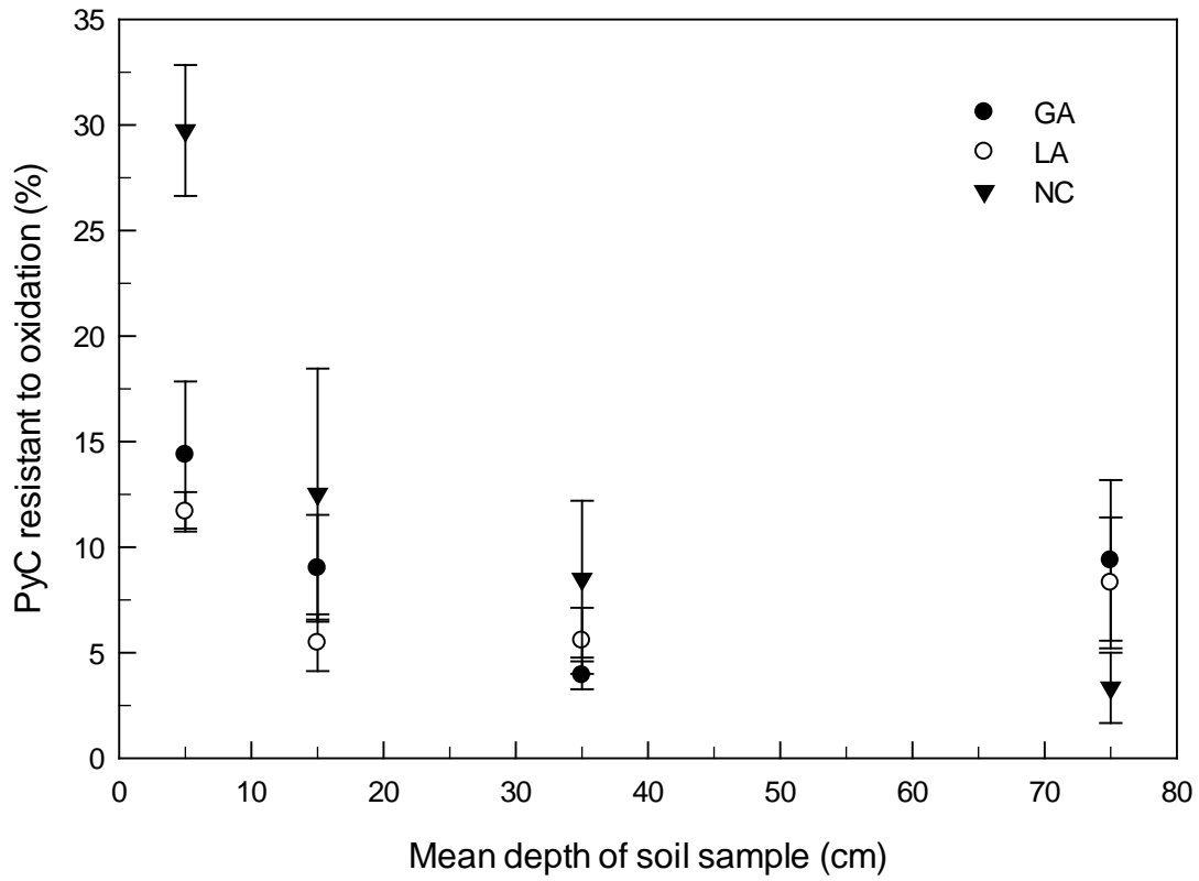
Figure 8.2. Percent of PyC resistant to oxidation with H_2O_2 and HNO_3 (+/- se.) from 14 longleaf pine stands in Georgia (n=5), Louisiana (n=5) and North Carolina (n=4) by depth.
