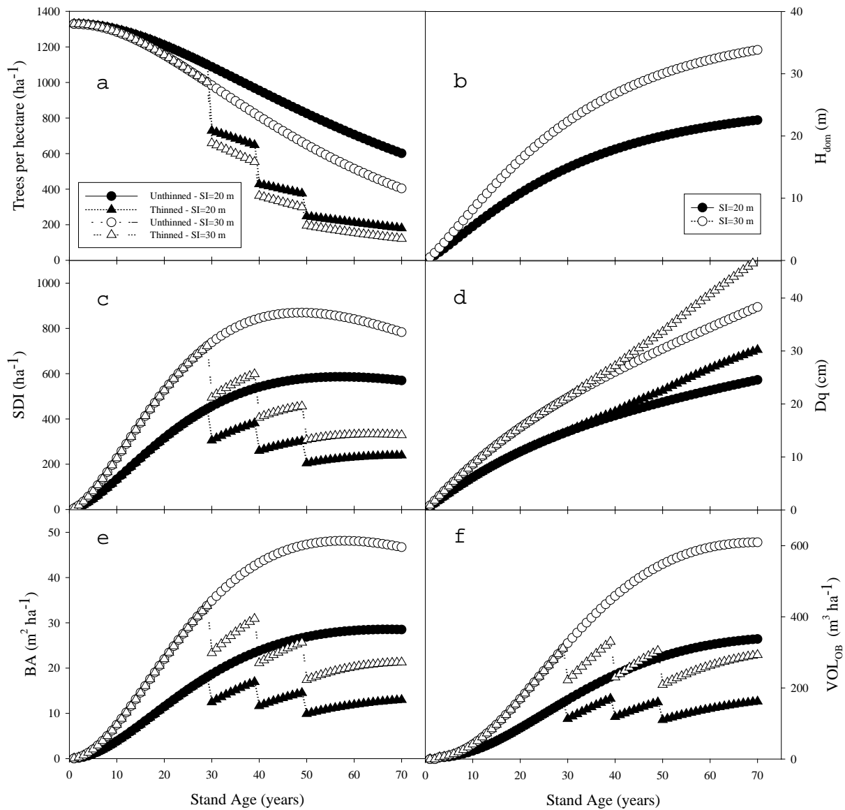
Figure 12.7 Example of model outputs. Simulation of survival (N, trees ha -1 ): (a) dominant height (H dom , m); (b) stand density index (SDI, trees ha -1 ); (c) quadratic mean diameter (Dq, cm); (d) basal area (BA, m 2 ·ha -1 ); (e) and stem volume outside bark (VOL OB , m 3 ·ha -1 ); (f) of unthinned (circle) and thinned (triangle) longleaf pine stands growing in sites with two different SI (20 m: black filled; 30 m: white filled).
