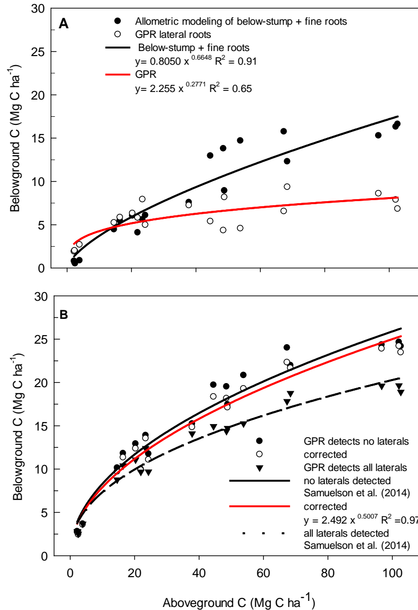
Figure 6.7. Comparison of above and belowground C from 20 plots of longleaf pine aged 5 to 87 years in Georgia (Samuelson et al. 2014) where lateral root C (GPR) is presented separate from below-stump C plus fine roots (allometric modelling) (A). Stand-level lateral root C (GPR) and below-stump mass plus fine roots (allometric modelling) were combined to calculate total root C (B). These data were originally reported by Samuelson et al. (2014) with assumptions of no lateral roots are detected by GPR in the below-stump sample area and all lateral roots are detected by GPR in the below-stump sample area . The lateral root (GPR) C data were corrected for below-stump underestimation using the approach and equation described in the present study.
