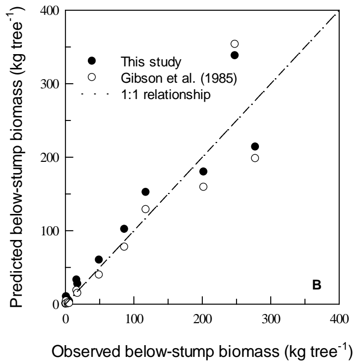
Figure 5.2. Observed versus predicted aboveground (A) and belowground (B) biomass using equations from this study and from other longleaf pine studies. The broken line represents the 1:1 relationship.
