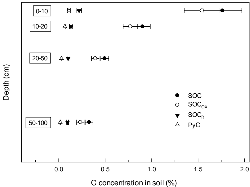
Figure 8.1. Concentration of SOC, SOC OX , SOC R and PyC in soil (+/- se.) from 14 longleaf pine stands in Georgia, Louisiana and North Carolina by sample depth.
