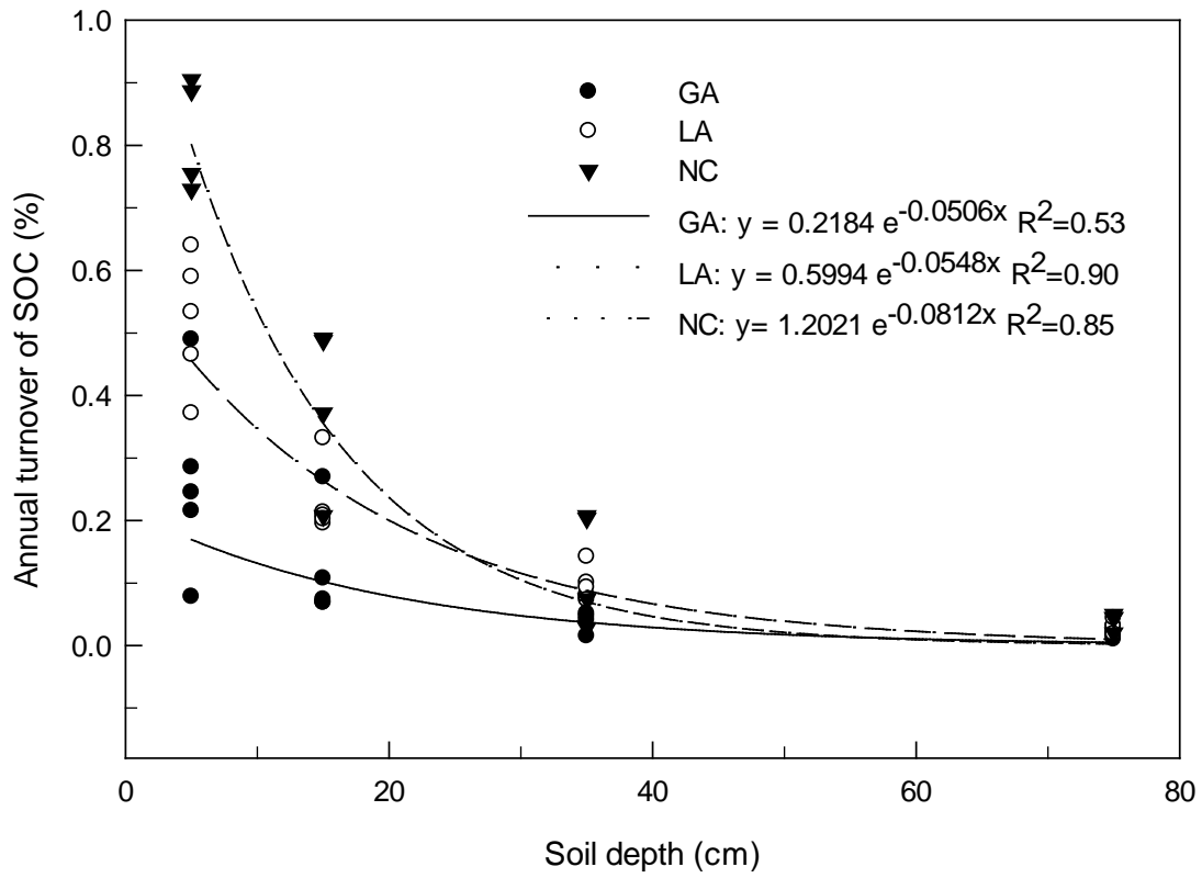
Figure 8.4. Annual turnover of SOC (%) from 14 longleaf pine stands in Georgia (n=5), Louisiana (n=5) and North Carolina (n=4) by depth.
