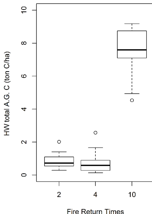
Figure 16.20. Mean simulated hardwood living above-ground carbon mass after 250 years of post-plantation management. Results are for fire return times of 2, 4, and 10 years.
