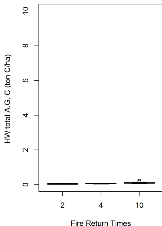
Figure 16.19. Mean simulated hardwood living above-ground carbon mass after 50 years of post-plantation management. Results are for fire return times of 2, 4, and 10 years.
