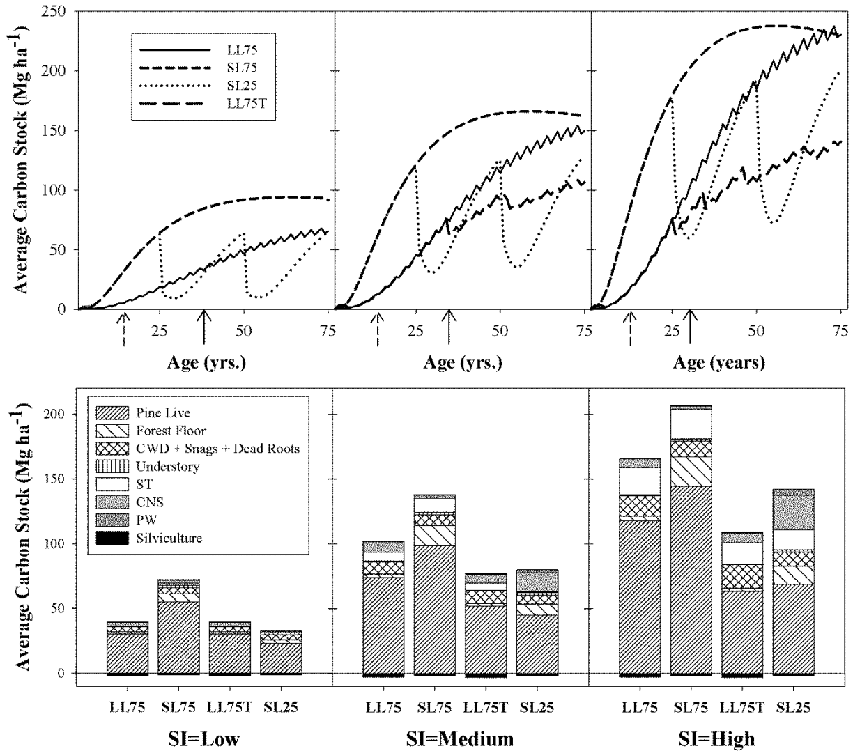
Figure 14.6. Average C stock for unthinned 75 year rotation longleaf (LL75) and slash (SL75), thinned 75 year rotation longleaf (LL75T) and unthinned 25 year rotation slash (SL25) pine plantations growing under three different site qualities (site index low, medium and high). Upper panel shows the dynamics of average C stock for the first 75 years. Arrows indicate year when current annual increment in average C stock peaked for SL75 (dashed) and LL75 (solid). Lower panel shows average C stock for a 300-year simulation period (4 rotations of 75 years for LL75, SL75 and LL75T, and 12 rotations of 25 years for SL25) (CWD: coarse woody debris; ST: sawtimber; CNS: chip-and-saw; PW: pulpwood).
