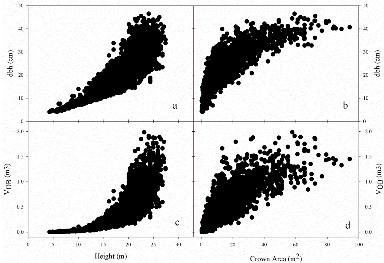
Figure 11.1. Relationships between total tree height ( H ) and crown area ( CA ) with stem diameter outside bark at 1.37 m height ( dbh ) (a, b) and stem volume outside bark ( V_{OB} ) (c, d) for the model development dataset.
