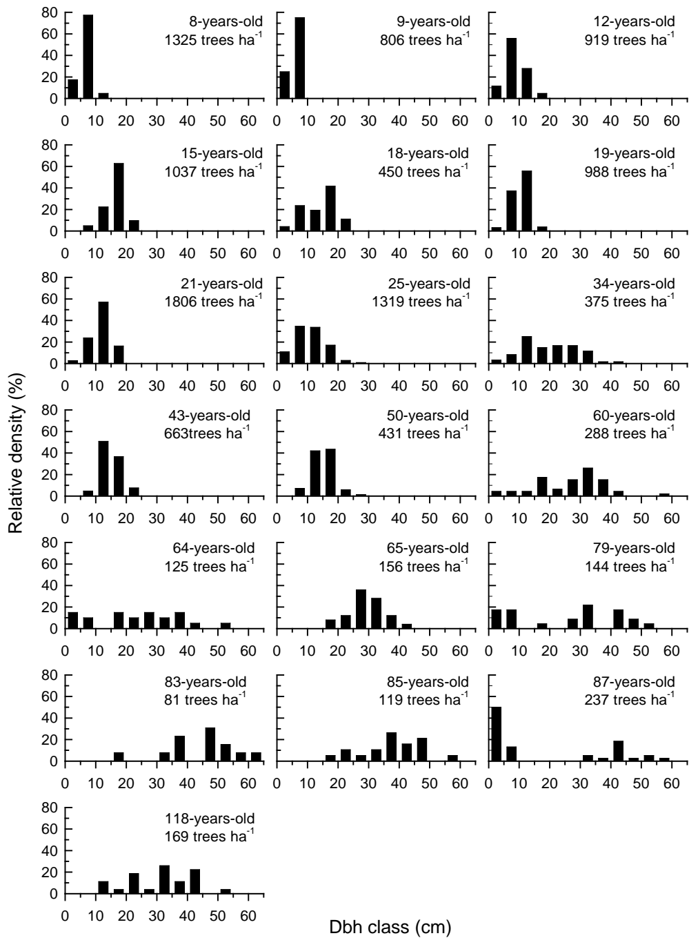
Figure 7.2. Diversity of forest structure in sampled loblolly pine stands.
