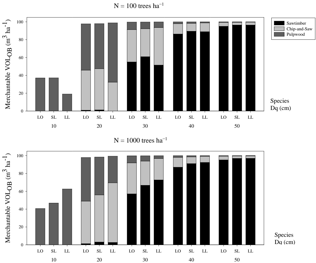
Figure 12.5. Comparison of merchantable volume yield breakdown functions published for P. taeda (LO, Harrison and Borders, 1996), P. elliotii (SL, Pienaar et al., 1996) and P. palustris (LL, this study). Effect of Dq (from 10 to 50 cm) and stand density [N = 100 trees ha -1 , upper panel (a); N = 1000 trees ha -1 , lower panel (b)] on volume yield breakdown for three product classes (sawtimber: d = 29.2 cm and t = 20.3 cm; chip-and-saw: d = 21.6 cm and t = 11.4 cm; pulpwood: d = 11.4 cm and t = 5.1 cm), assuming a VOL OB of 100 m 3 ·ha -1 .
