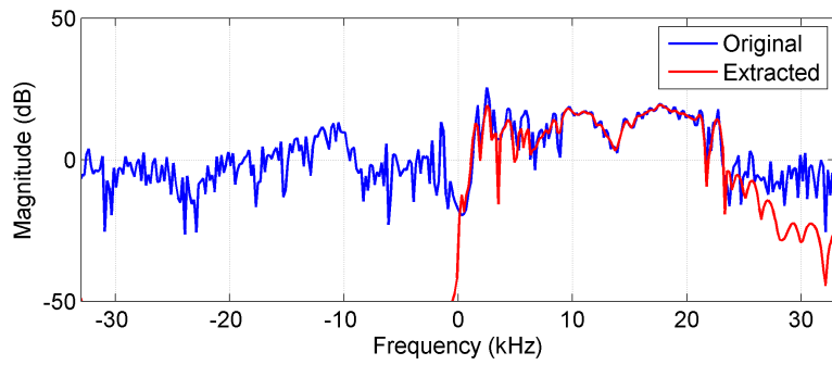
(b) The same signals as in (a), in frequency domain
