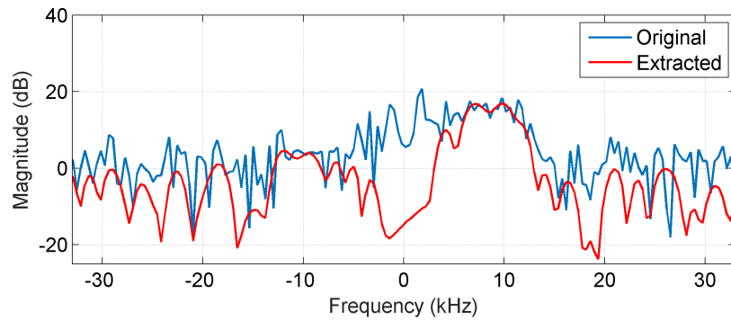
(b) The same signal as above, in frequency domain
