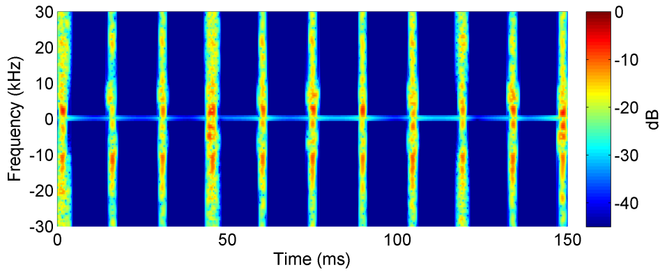
(b) Extracted tail signal
