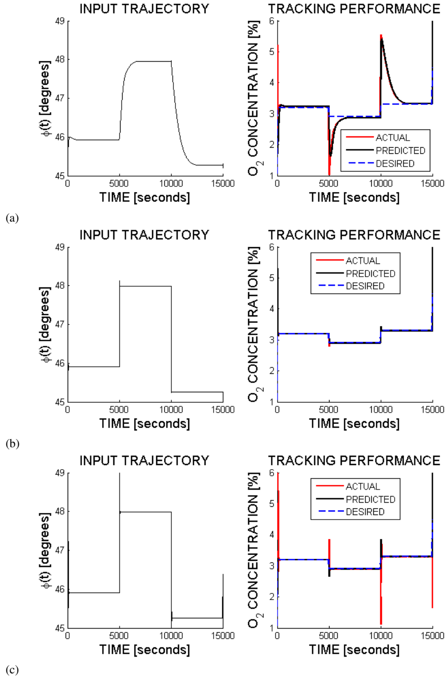
Figure 4.3: Case 1 Results—Step Tracking. The reference input was tracked using Neural GPC (a), SBMPC RBF (b), and SBMPC BPN (c). The neural network type affects overshoot due to larger BPN prediction errors. SBMPC convergence, however, is still more rapid than that of GPC regardless of neural network choice.
