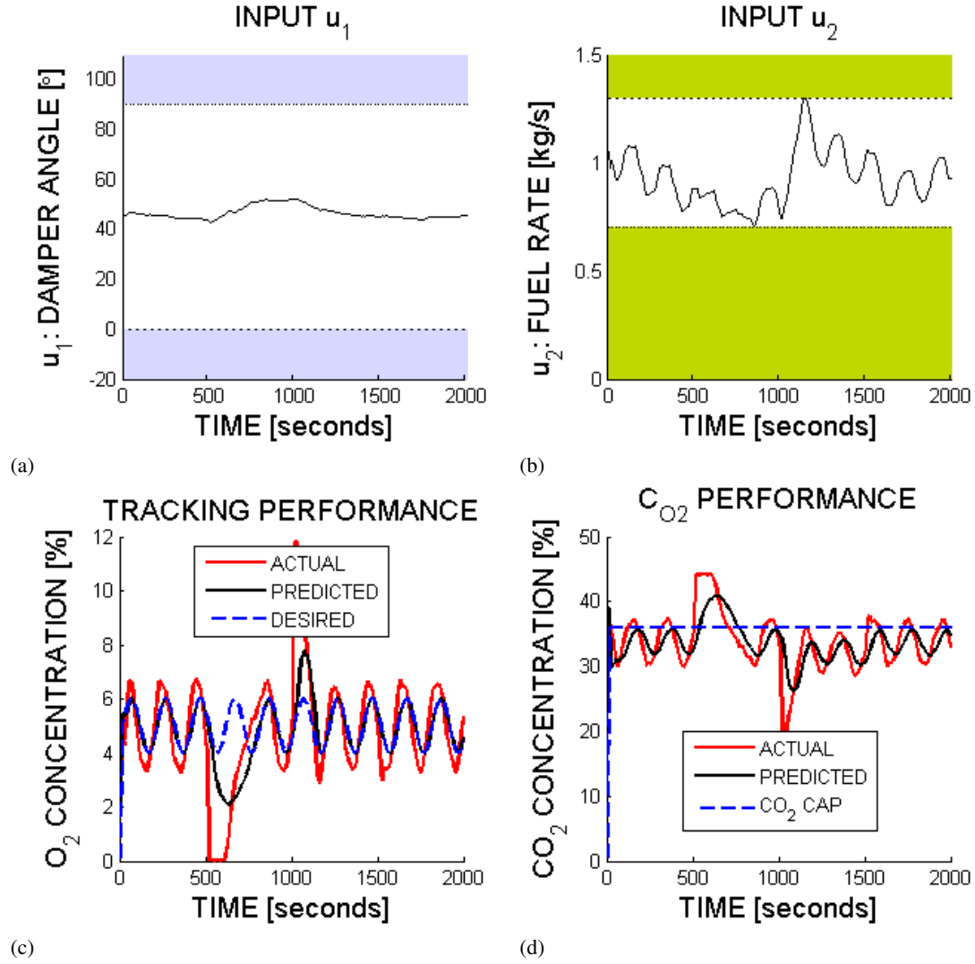
Figure 4.9: SBMPC BPN Case 3 Results. SBMPC BPN adapts to the plant changes at 500 second intervals. Plots of inputs dampener angle (a) and fuel rate (b), and outputs oxygen concentration (c) and carbon dioxide concentration (d) are given. The shaded upper and lower regions on the input plots are infeasible regions beyond the input constraints.
