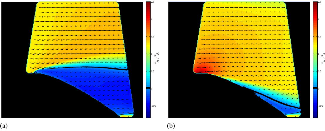
Figure 5.32: Baseline (a) and Controlled (b) V_x for 22°, 12 m/s. The baseline PIV data was collected with the control system off. In the controlled case, data was collected with the control system set to maximize Z_{lift} , and the tunnel speed corresponds to a Reynolds number of 125,000 based on chord length.
