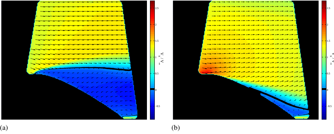
Figure 5.31: Baseline (a) and Controlled (b) V_x for 22°, 11 m/s. The baseline PIV data was collected with the control system off. In the controlled case, data was collected with the control system set to maximize Z_{lift} , and the tunnel speed corresponds to a Reynolds number of 90,000 based on chord length.
