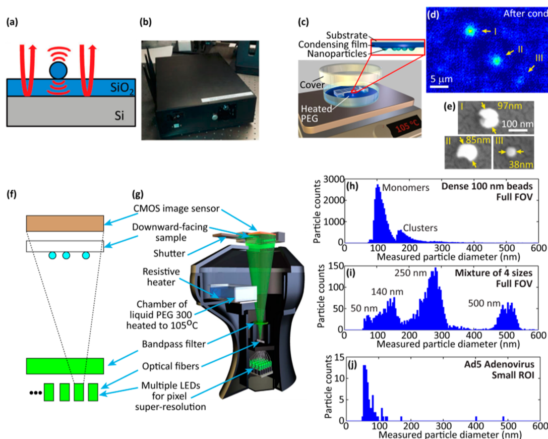
Figure 4. Interferometric imaging and sizing of nanoparticles. (a) Single particle interferometric reflectance imaging sensing (SP-IRIS) scheme. The signal is generated from the interference between the scattered light from the particle and the light reflected from the SiO 2 –Si interface. (b) Portable prototype capable of SP-IRIS sensing at the point of care. (c–j) Imaging and sizing of nanoparticles using lensfree holographic on-chip imaging. (c) The condensation of polyethylene glycol (PEG) vapor can be used to form nanolenses that increase the scattering signatures from embedded nanoparticles and enable their detection. (d) Nanoparticles smaller than 40 nm are visible after PEG condensation. (e) Scanning electron microscopy gold-standard comparisons for the particles in (d). (f, g) Line drawing and schematic of a “democratic” nanoscale measurement tool incorporating nanolens formation and imaging. Note that the optical fibers in this design are multimode and rather easy to couple light through simple butt coupling. (h–j) Nanoparticle sizing histograms obtained using the device shown in (g). Panel (a) reproduced from Daaboul, G. G.; Yurt, A.; Zhang, X.; Hwang, G. M.; Goldberg, B. B.; Ünlü, M. S. Nano Lett. 2010 , 10 , 4727–4731 (ref 70). Copyright 2010 American Chemical Society. Panel (b) is reprinted with permission from Reddington, A. P.; Trueb, J. T.; Freedman, D. S.; Tuysuzoglu, A.; Daaboul, G. G.; Lopez, C. A.; Karl, W. C.; Connor, J. H.; Fawcett, H.; Unlu, M. S. IEEE Trans. Biomed. Eng. 2013 , 60 , 3276–3283 (ref 72). Copyright 2013 Institute of Electrical and Electronics Engineers. Panels (c–e) reproduced from McLeod, E.; Nguyen, C.; Huang, P.; Luo, W.; Veli, M.; Ozcan, A. ACS Nano 2014 , 8 , 7340–7349 (ref 84). Copyright 2014 American Chemical Society. Panels (g–j) reproduced from McLeod, E.; Dincer, T. U.; Veli, M.; Ertas, Y. N.; Nguyen, C.; Luo, W.; Greenbaum, A.; Feizi, A.; Ozcan, A. ACS Nano 2015 , 9 , 3265–3273 (ref 69). Copyright 2015 American Chemical Society.
