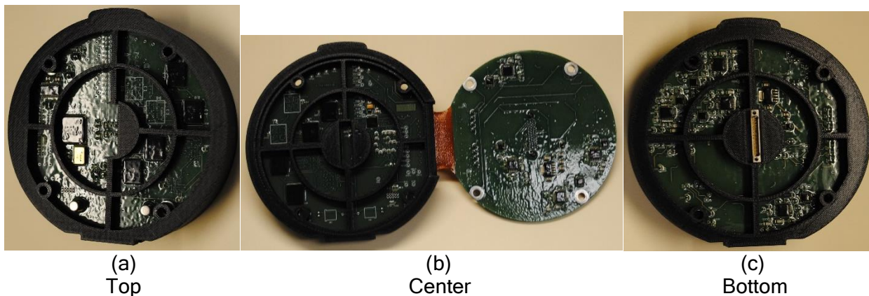
Figure 19 PCB spacers
