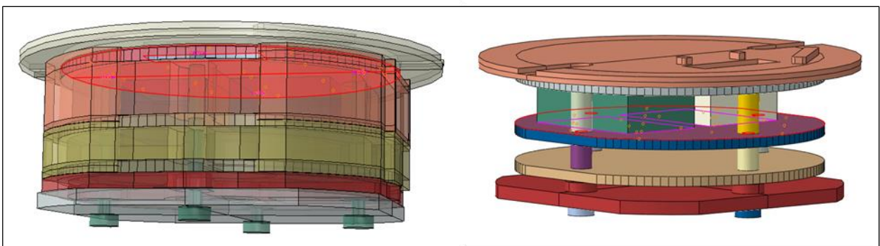
Figure 22 Tie constraints are identical for all three models
