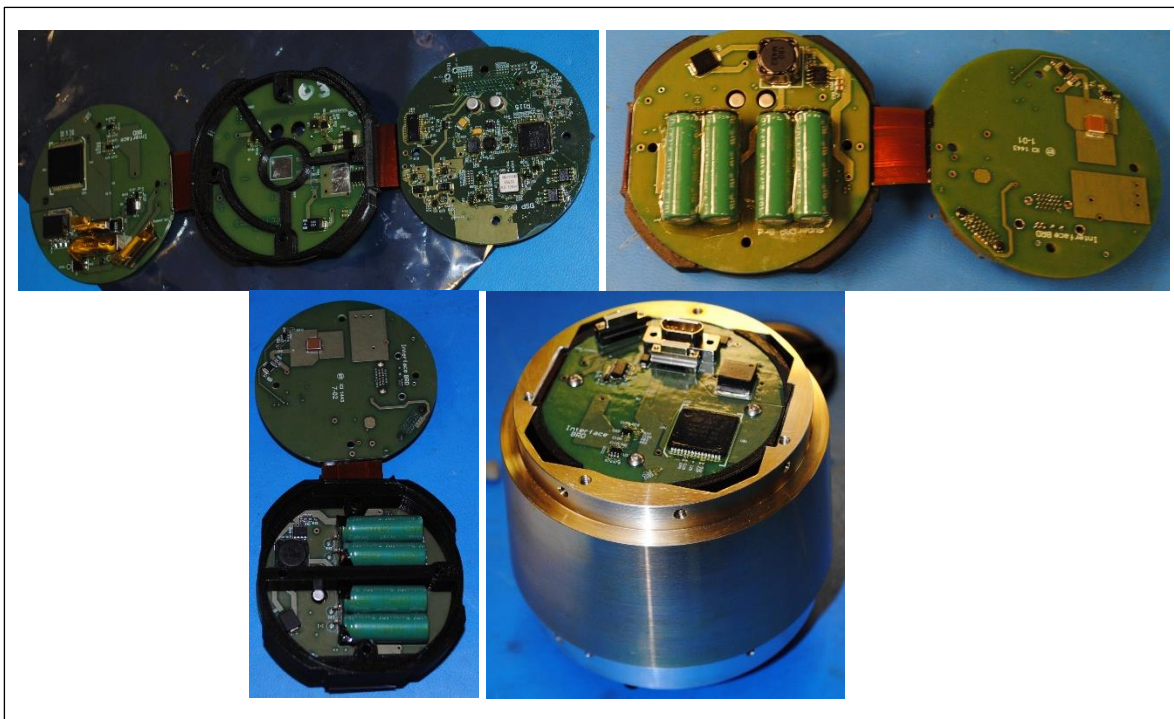
Figure 24 GEU assembly photos
