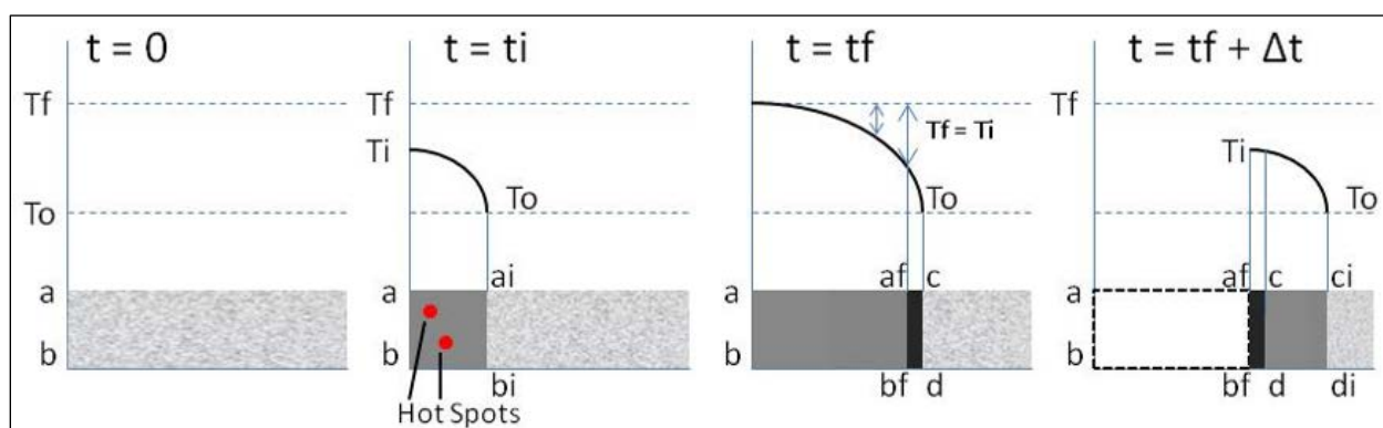
Figure 1. Pictorial representation of Shimizu's hypothesis, which was adapted from his 1982 article (1). Here, temperature ( T ) is shown as a function of time ( t ), with T_0 as the initial temperature at the beginning of the dark phase and T_i as the temperature of the burning layer. Ignition occurs on the composition's surface ( ab ). When the temperature ( T_i ) of the layer ( aba_i b_i ) reaches the flash reaction temperature ( T_f ), the layer ( aba_f b_f ) becomes consumed by flash. The temperature then drops, and it results in the formation of a thin layer ( a_f b_f c d ) on the surface ( cd ), which will initiate the next dark phase.
