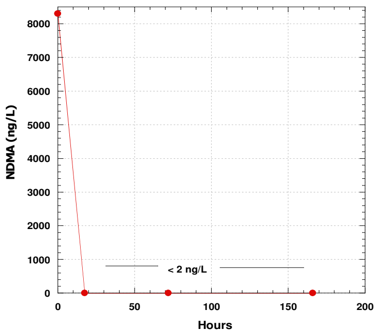
Figure 2-3. Biodegradation of NDMA by the propanotroph Rhodococcus ruber ENV425 in batch culture. Propane was added to the headspace of the reaction vessel. NDMA levels were below the PQL of 2 ng/L after 18 hr.
