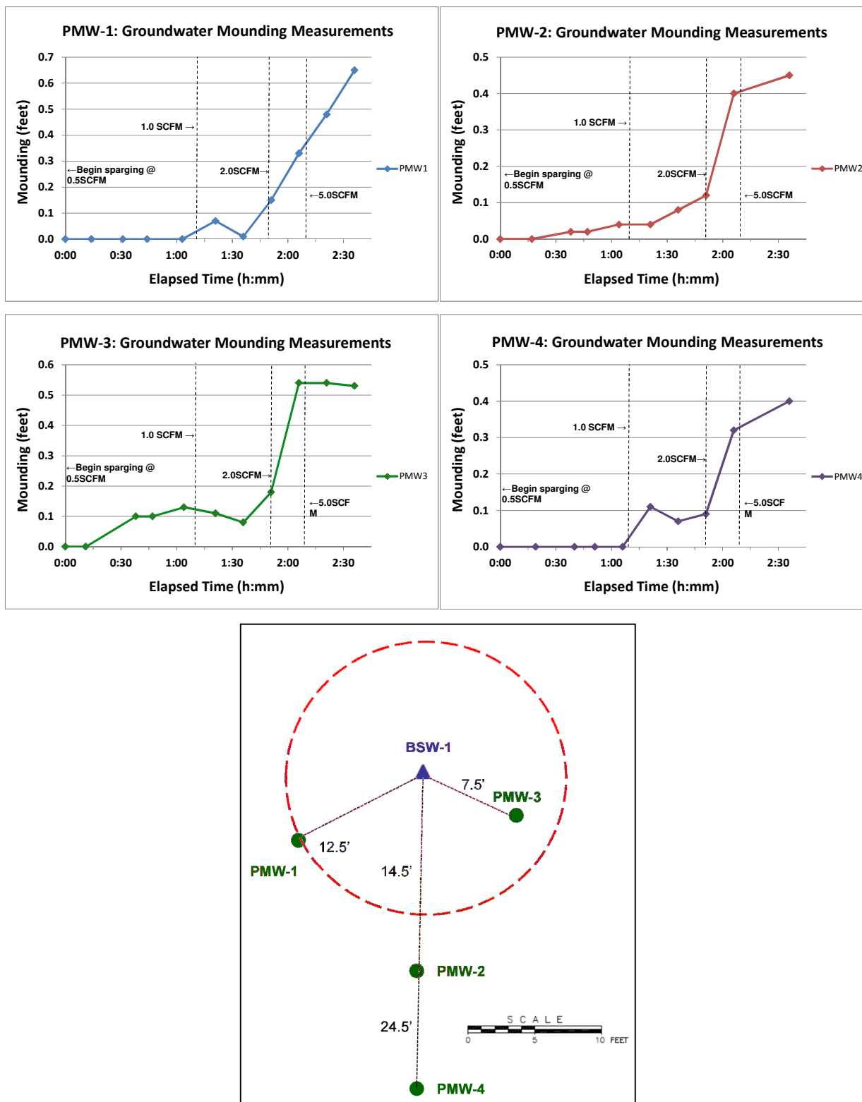
Figure 5-1. Groundwater mounding measurements in PMW-1 to PMW-4 during air sparge testing at BSW-1. The air flow rates are provided for each well and a view of the approximate well locations is provided in the bottom panel.
