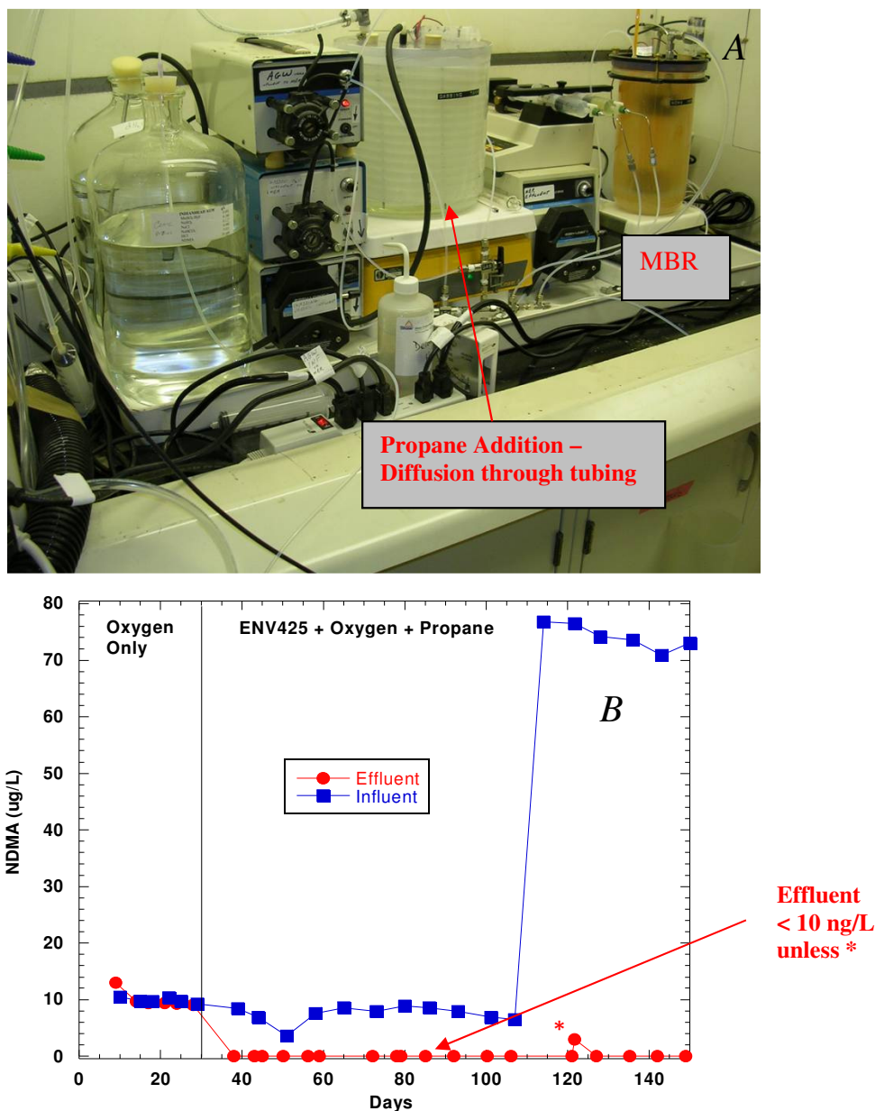
Figure 2-6. Laboratory propane-fed membrane bioreactor treating NDMA (Panel A). Influent and effluent data from the MBR (Panel B). All effluent points after culture inoculation were < 10 ng/L except that denoted with a *. Modified from Hatzinger et al., (2011).
