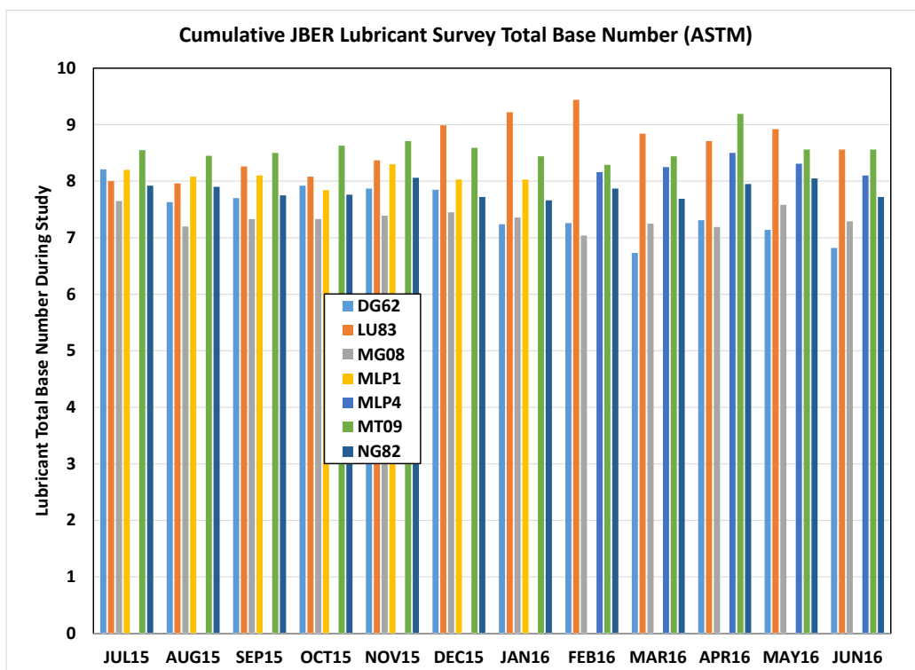
Figure 19. Asset ASTM D4739 Total Base Number for Study at JBER
