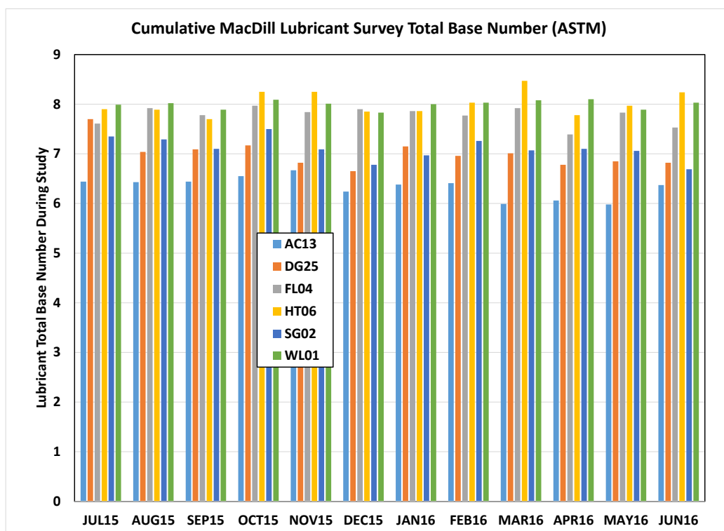
Figure 22. Asset ASTM D4739 Total Base Number for Study at MacDill
