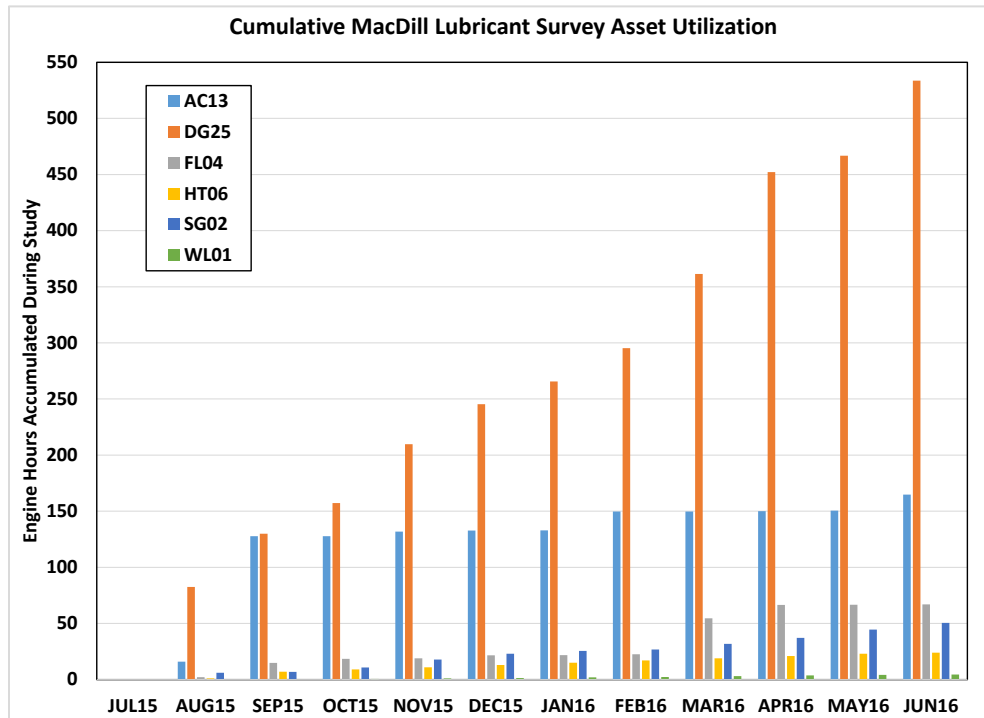
Figure 17. Operational Hours Accumulated by Assets During Study at MacDill
