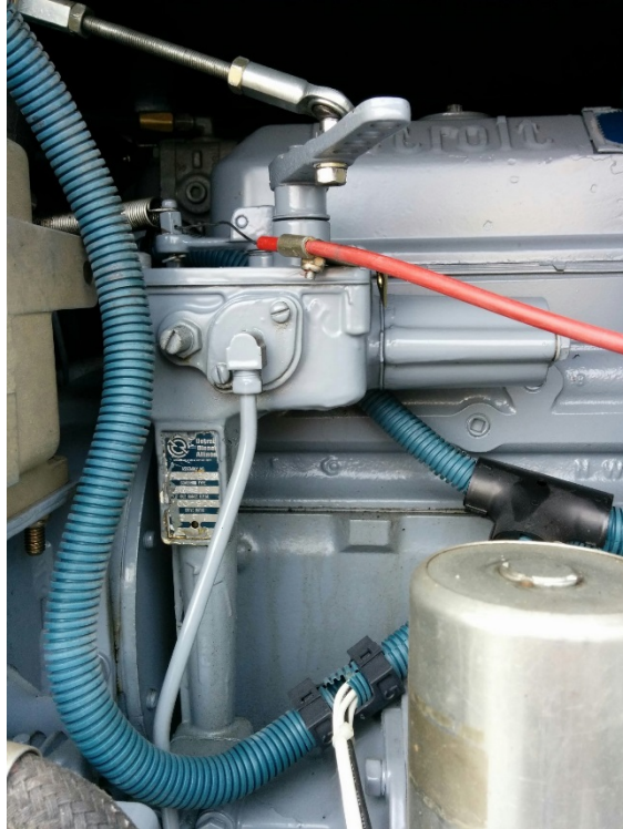
Figure 3. Detroit Diesel Engine from MG08 Model A/M32A-86D Generator at JBER
