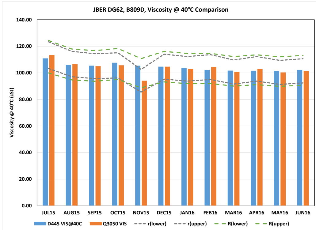
Figure 27. Comparison of ASTM and Portable Viscosity @ 40 °C for JBER DG62 Asset
