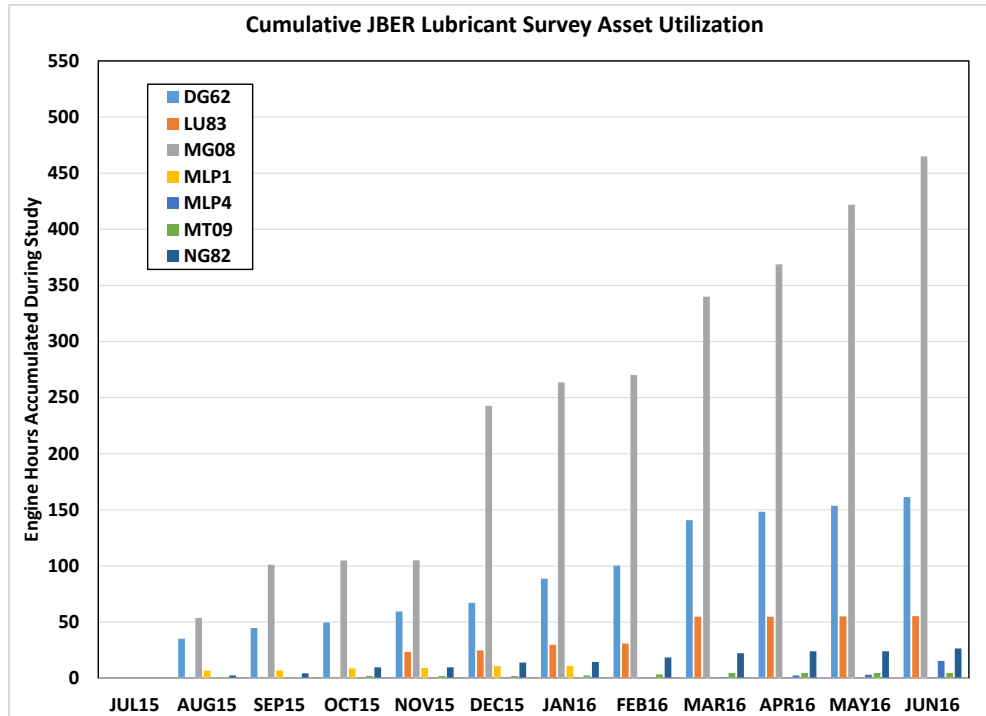
Figure 16. Operational Hours Accumulated by Assets During Study at JBER
