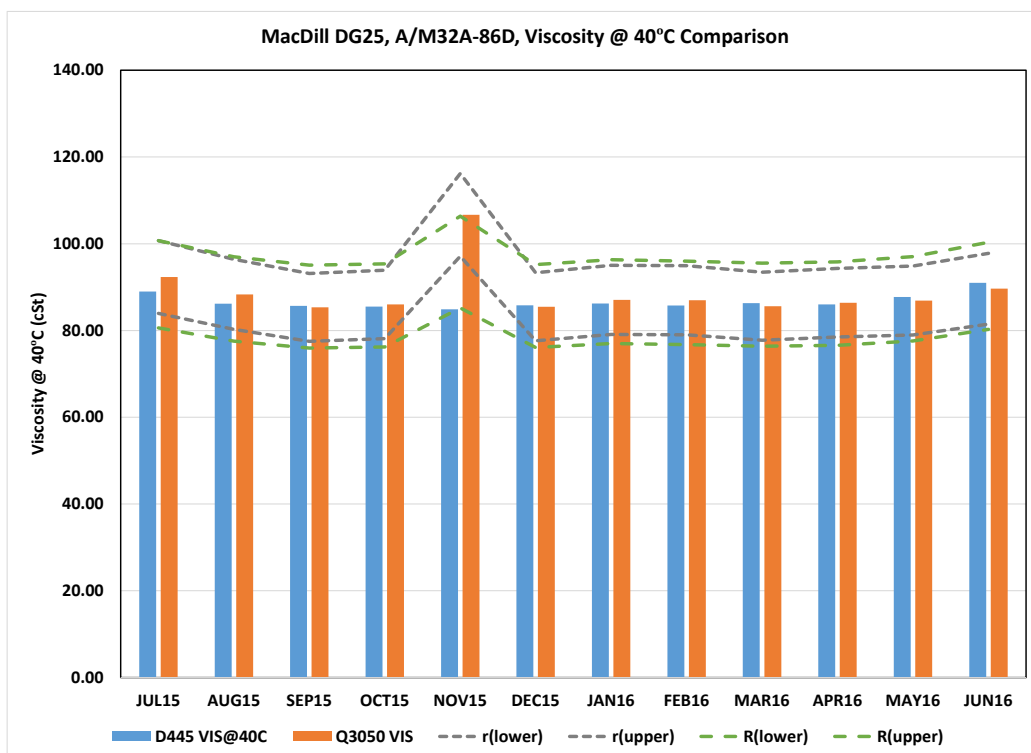
Figure 31. Comparison of ASTM and Portable Viscosity @ 40 °C for MacDill DG25 Asset
