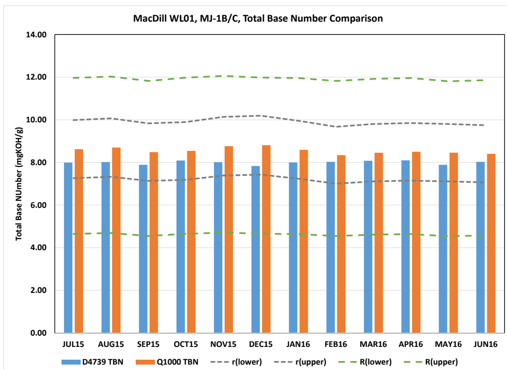
Figure 34. Comparison of ASTM and Portable Total Base Number for MacDill WL01 Asset
