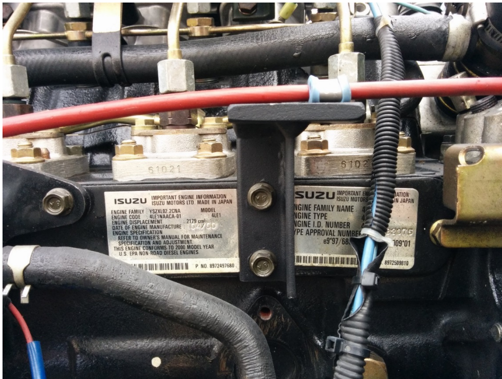
Figure 4. Isuzu 4LE1 Engine for SG62 Model SGNSC at JBER
