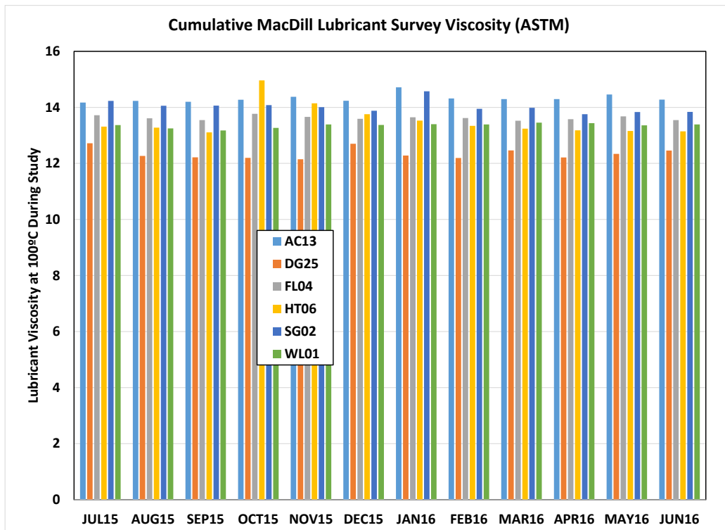
Figure 21. Asset ASTM D445 Viscosity at 100 °C for Study at MacDill
