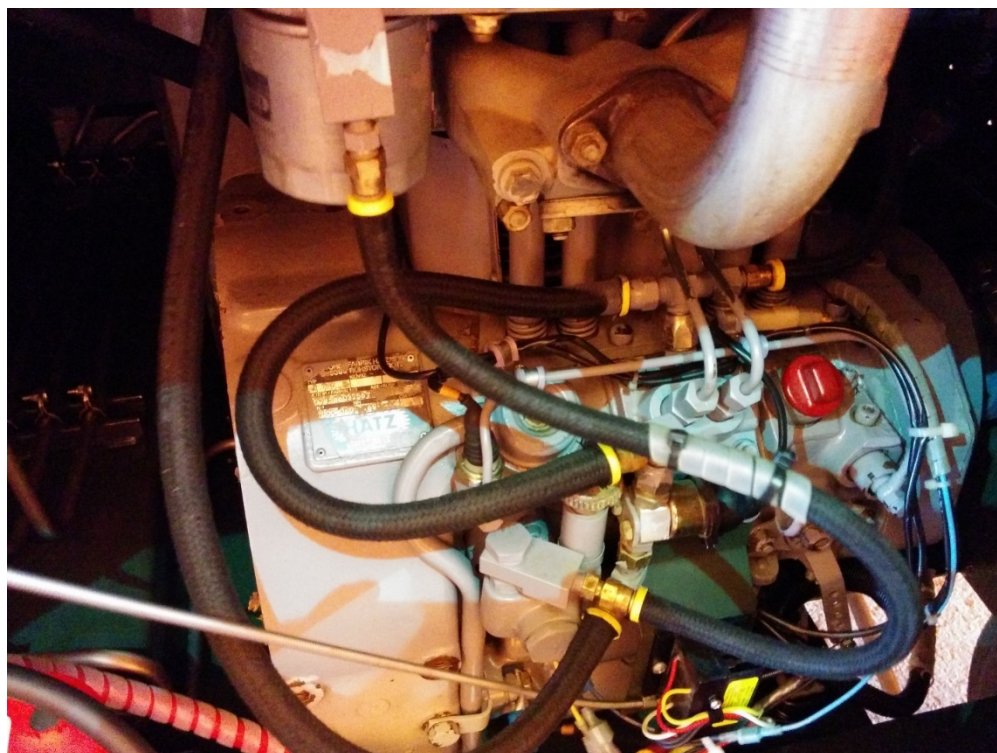
Figure 5. Hatz Engine for MT09 AF/M27M-1 Hydraulic Jacking Manifold at JBER
