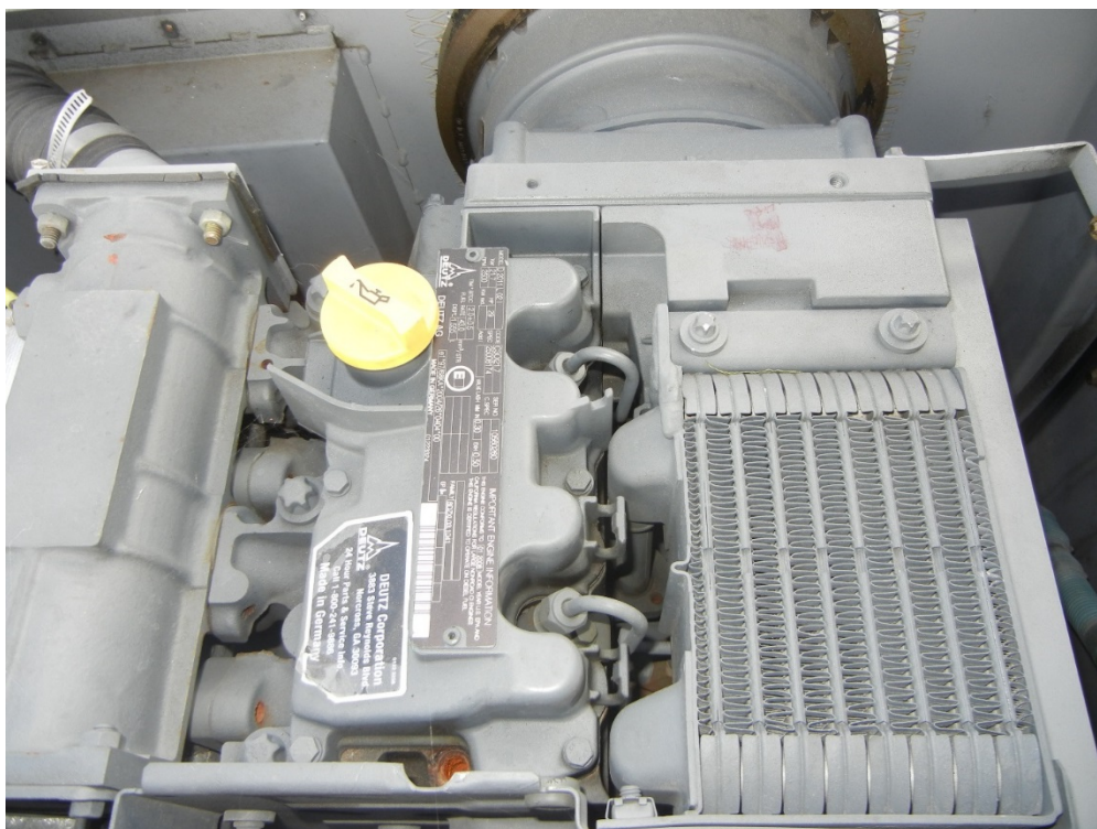
Figure 12. Deutz Engine from WL01 Model MJ-1B/C at MacDill AFB
