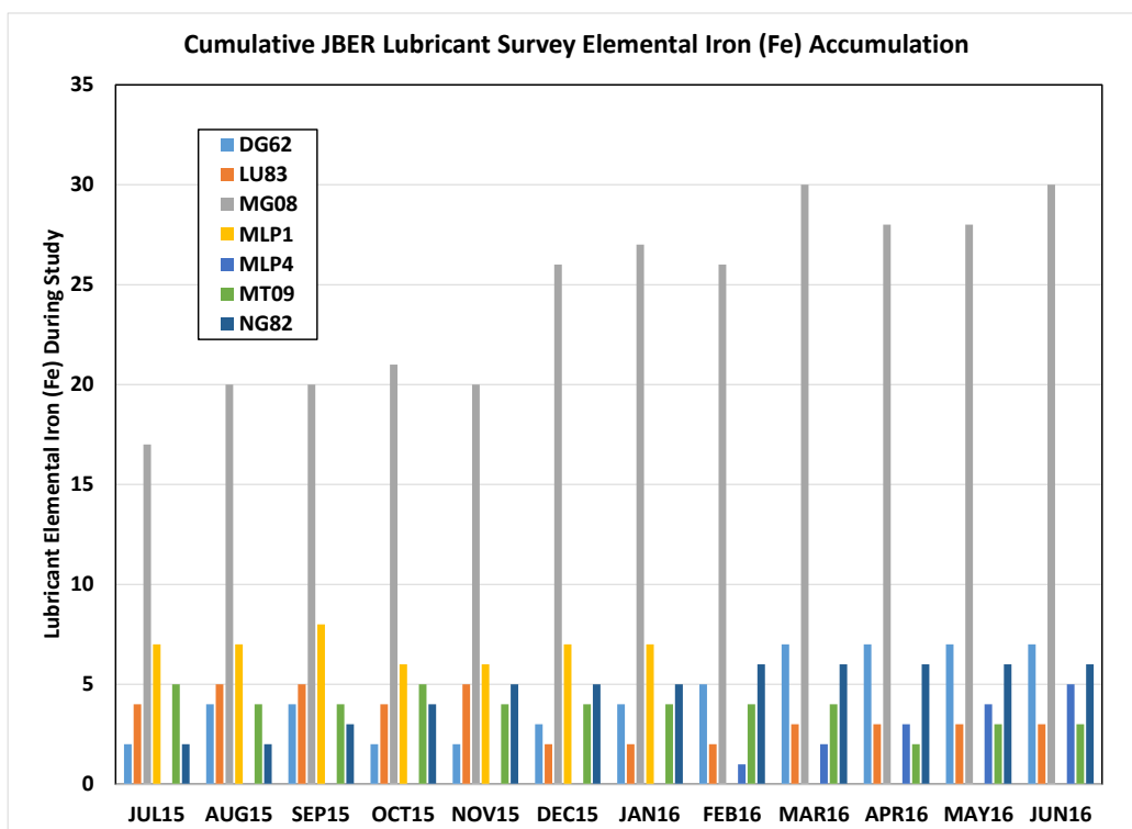
Figure 20. Asset ASTM D5185 Iron (Fe) Wear Element for Study at JBER
