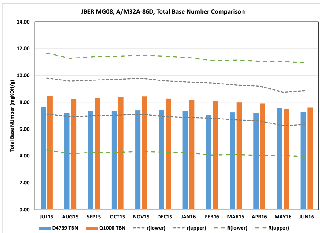
Figure 24. Comparison of ASTM and Portable Total Base Number for JBER MG08 Asset
