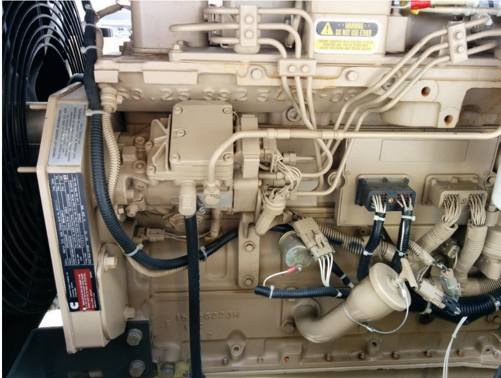
Figure 1. Cummins B5.9 Engine from DG62 Model B809D Generator at JBER
