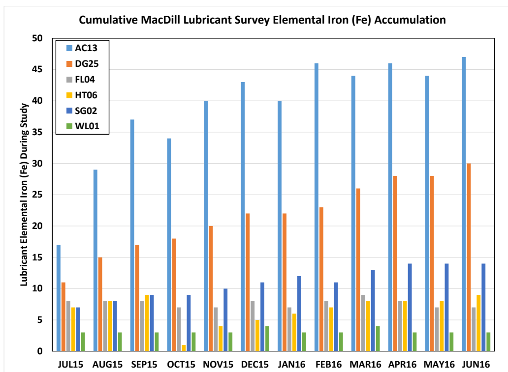
Figure 23. Asset ASTM D5185 Iron (Fe) Wear Element for Study at MacDill
