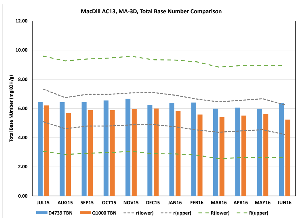
Figure 32. Comparison of ASTM and Portable Total Base Number for MacDill Asset AC13
