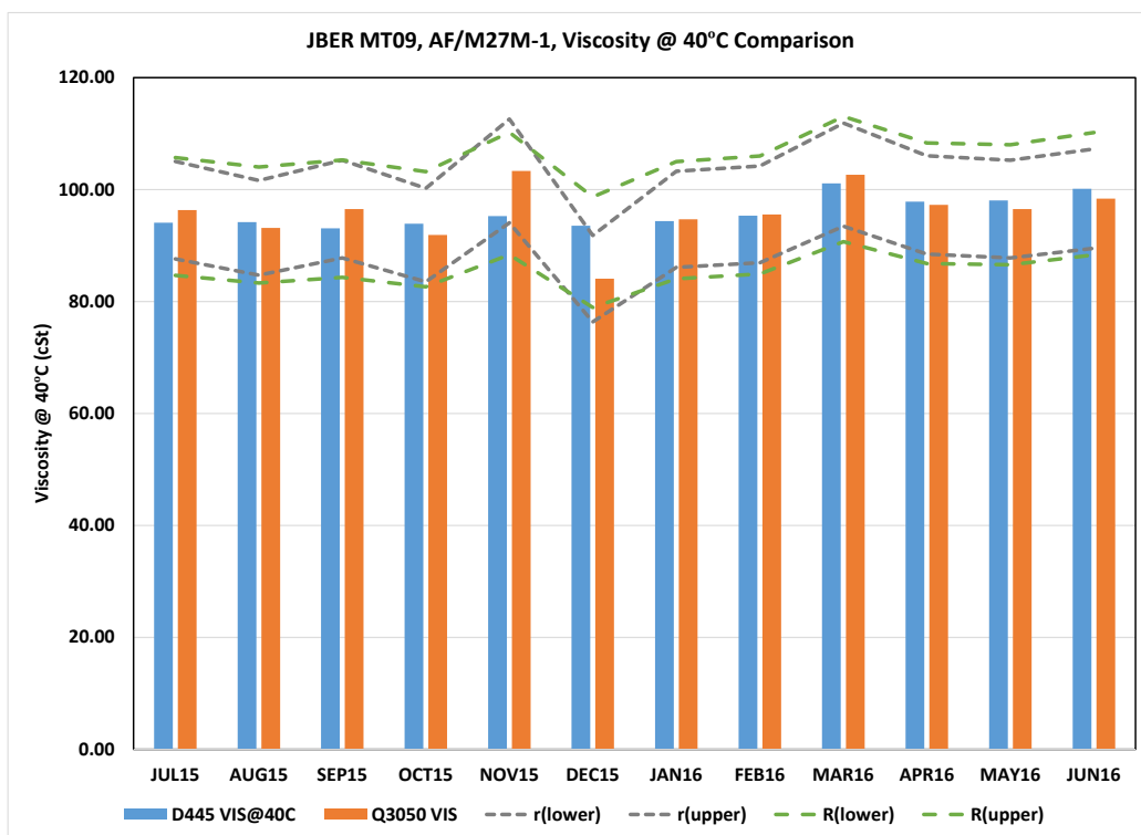
Figure 29. Comparison of ASTM and Portable Viscosity @ 40 °C for JBER MT09 Asset
