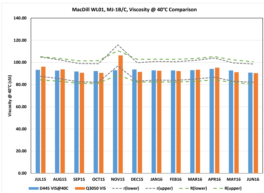
Figure 35. Comparison of ASTM and Portable Viscosity @ 40 °C for MacDill WL01 Asset
