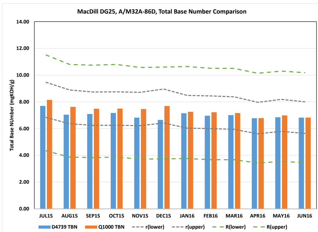
Figure 30. Comparison of ASTM and Portable Total Base Number for MacDill DG25 Asset
