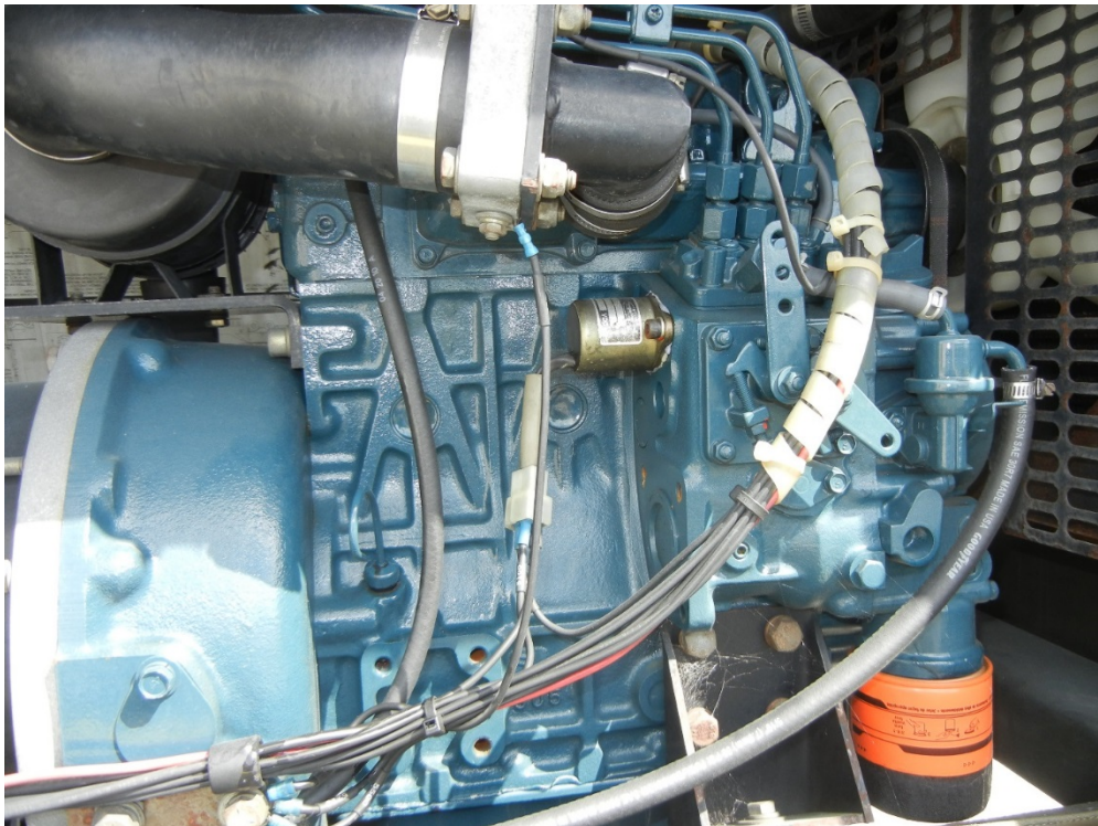
Figure 8. Kubota Engine for FL04 Model FL-1D Light Cart at MacDill AFB
