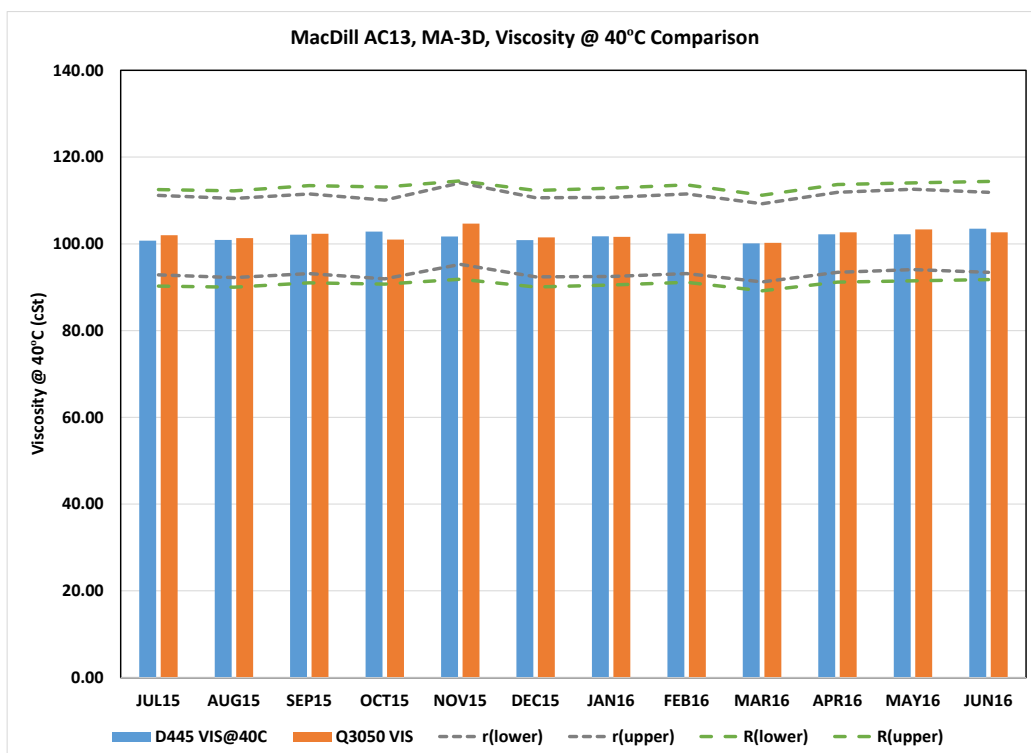
Figure 33. Comparison of ASTM and Portable Viscosity @ 40 °C for MacDill AC13 Asset
