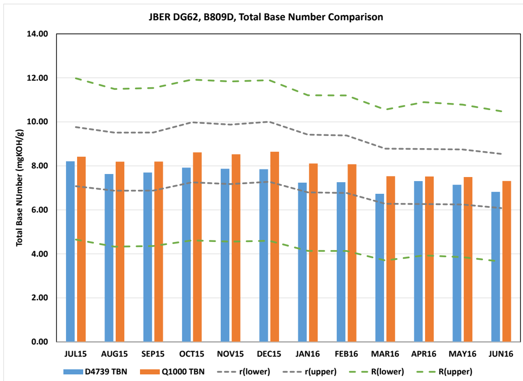
Figure 26. Comparison of ASTM and Portable Total Base Number for JBER DG62 Asset
