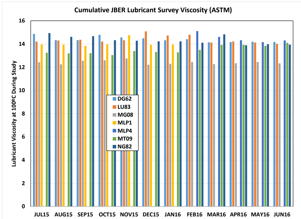
Figure 18. Asset ASTM D445 Viscosity at 100 °C for Study at JBER
