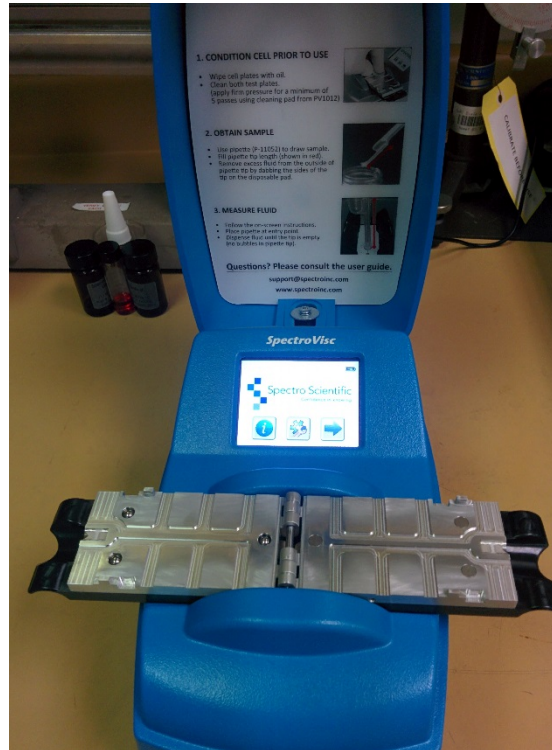
Figure 15. Sample Cell Micro-Channels of the SpectroVisc Q3050 Used for Viscosity Measurement
