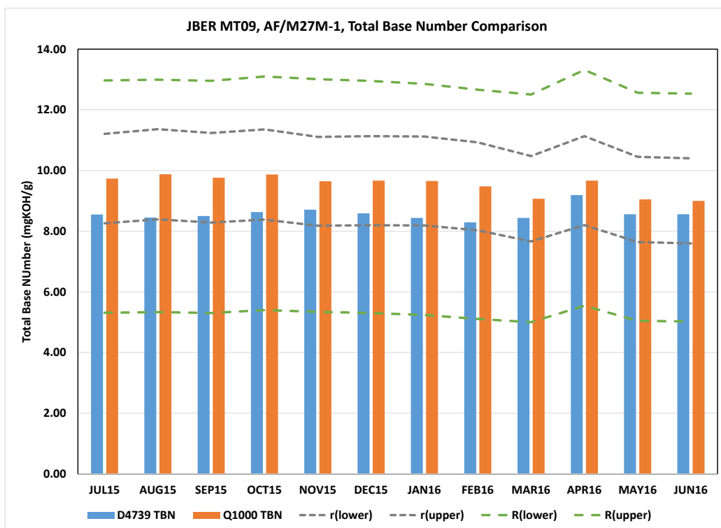
Figure 28. Comparison of ASTM and Portable Total Base Number for JBER MT09 Asset
