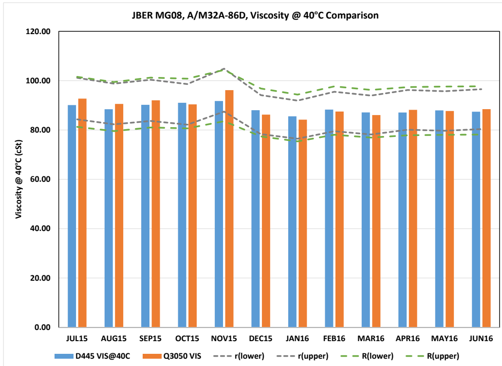
Figure 25. Comparison of ASTM and Portable Viscosity @ 40 °C for JBER MG08 Asset
