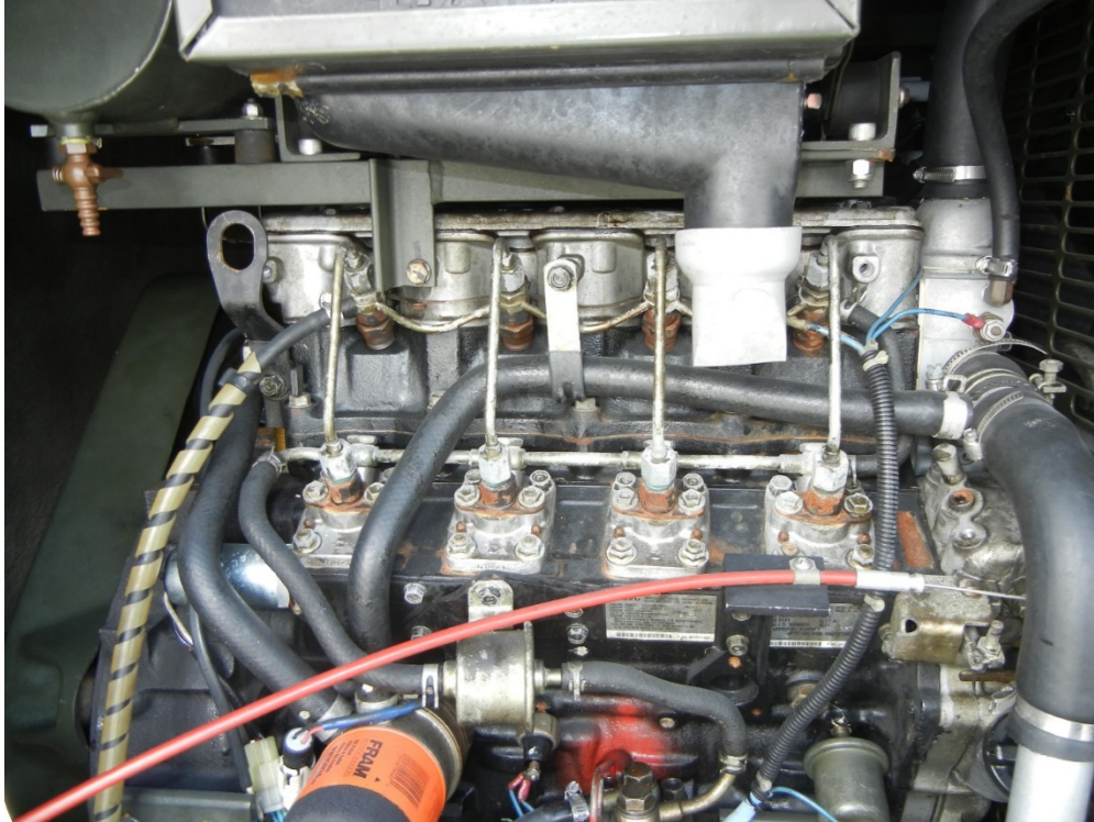
Figure 7. Isuzu 4LE1 Engine from SG02 Model SGNSC at MacDill AFB
