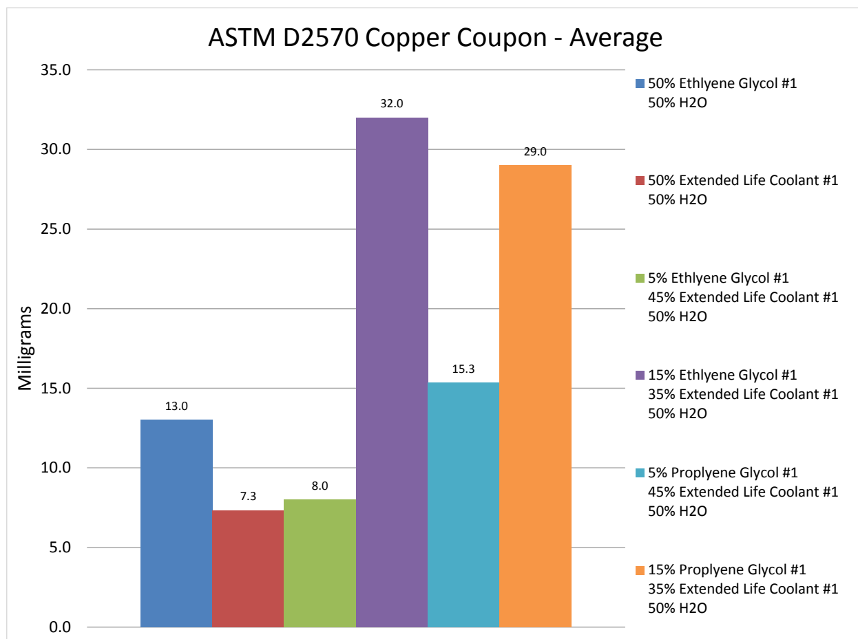
Figure 4. ASTM D2570 Copper Coupon Mass Loss
