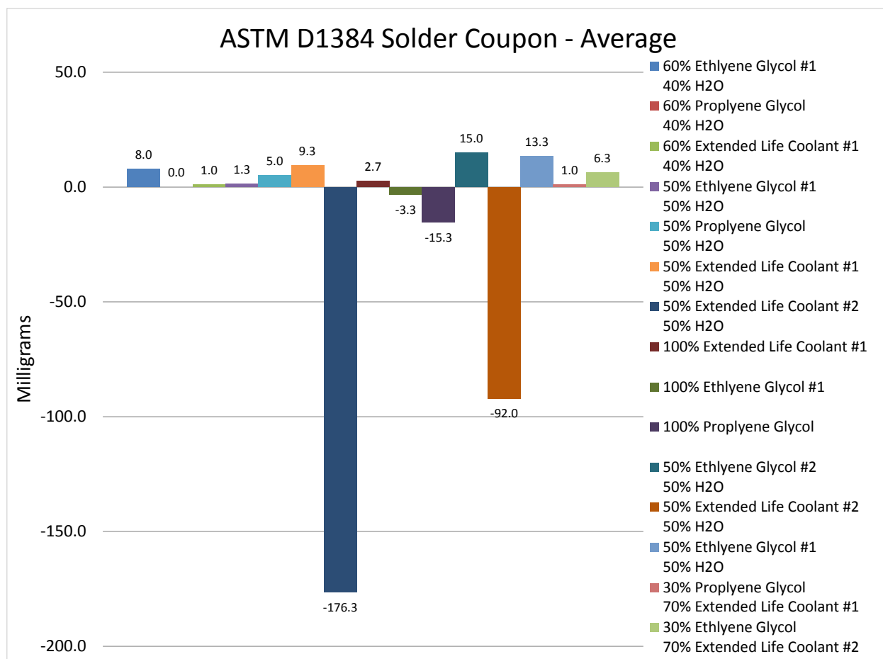
Figure 1. ASTM D1384 Solder Coupon Mass Loss
