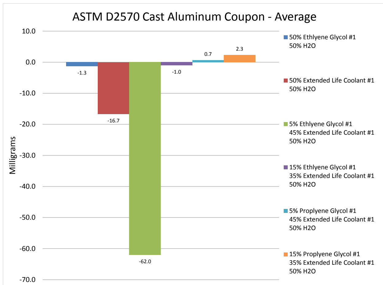
Figure 5. ASTM D2570 Cast Aluminum Coupon Mass Loss
