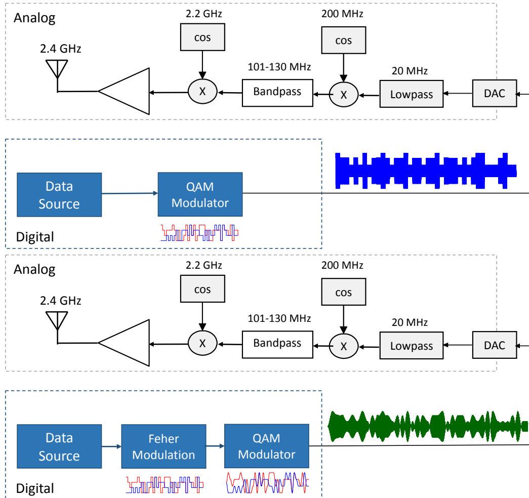
Fig. 19 Quadrature amplitude modulation software-defined radio example
