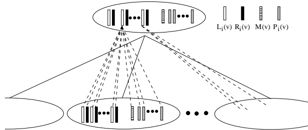
Figure 7: The virtual forest.
