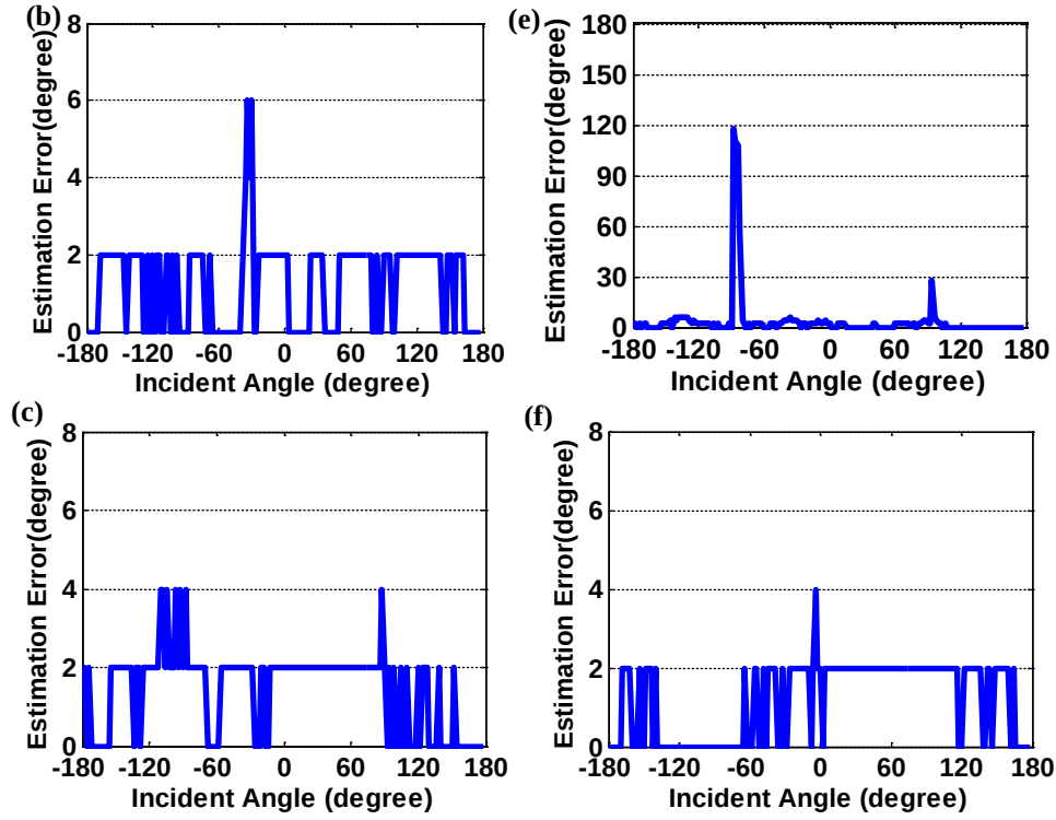
Figure 18. The measured estimation errors of the elliptical UWB antenna (left) and D-shaped antenna (right) respectively with the incident wave in (a, d) the x-y plane (with H-field in the z direction), (b, e) the x-z plane (with H-field in the y direction), and (c, f) the y-z plane (with E-field in the x direction).
