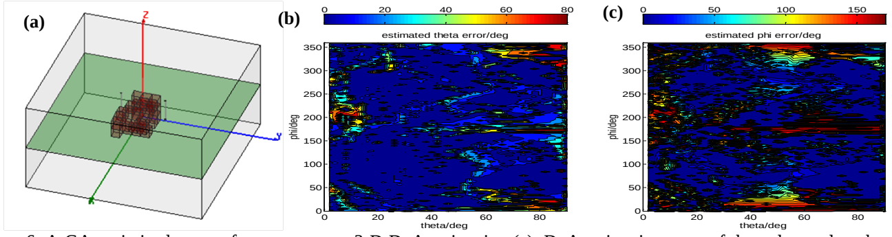
Figure 6. A GA optimized scatterer for two-antenna 3-D DoA estimation (a), DoA estimation error of the polar angle - theta (b) and of the azimuthal angle - phi (c)
