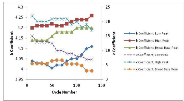
Figure 12. The “b” and “c” charge coefficients for the three-curve Gaussian model over the life cycle of a spinel button cell. The “b” coefficients correspond to the primary axis, and the “c” coefficients correspond to the secondary axis.
