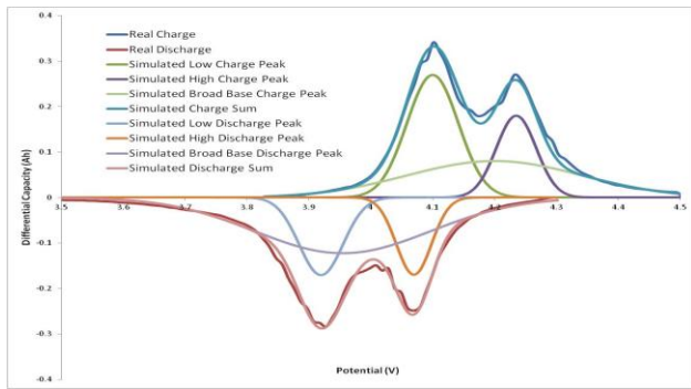
Figure 8. Differential capacity curve with its three-curve Gaussian model for a spinel button cell.
