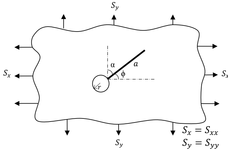
Figure 7: Cracked circular hole subjected to biaxial stresses.
