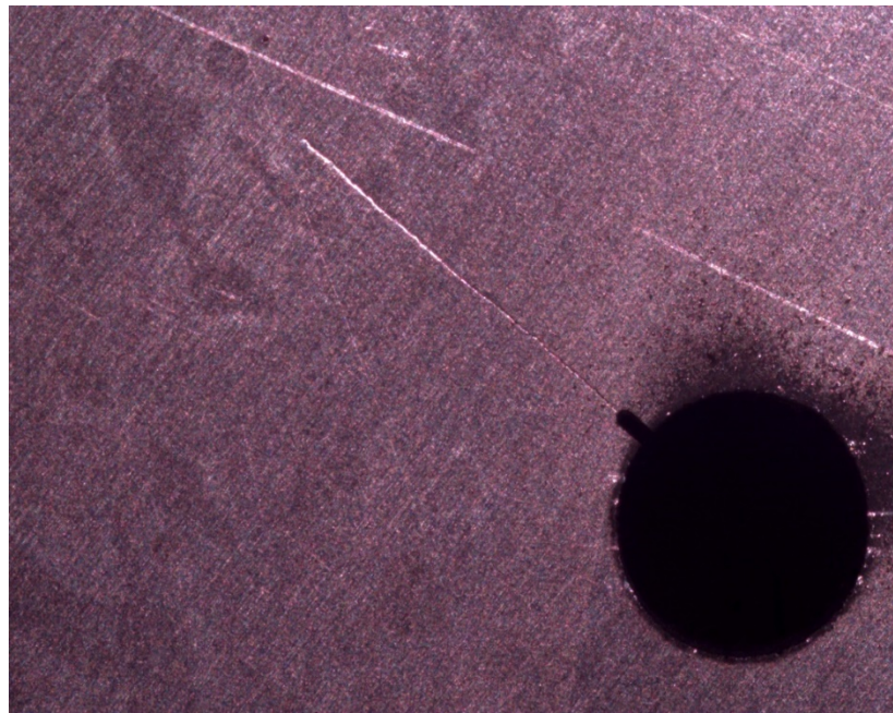
Figure 50: 13.33 mm crack length after 455,000 fatigue cycles at R=0.1 in air environment.
