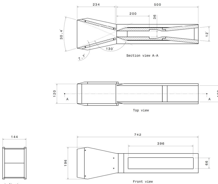
Figure 5 – 3 Views and a section of fundamental combustion experiment hardware
