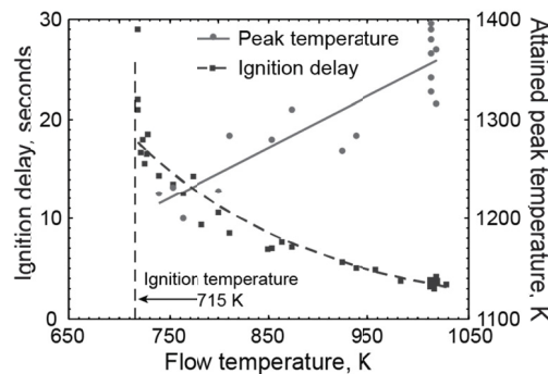
Figure 9 Delay times and maximum attained temperature before quenching of the first ignition stage for the crystalline boron agglomerates.
