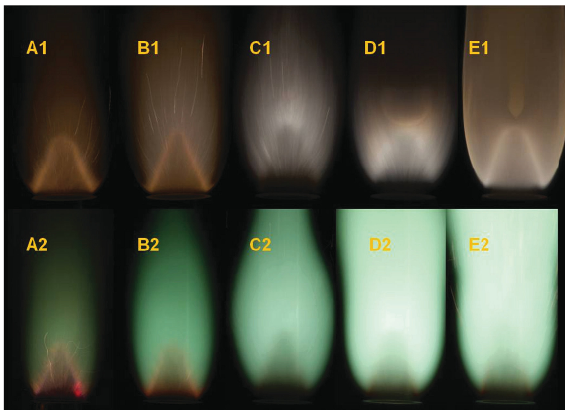
Figure 17. (top) progression of flame in a \text{CH}_4\text{-Al-26\% O}_2 flame from low concentration in A1 to high concentration in E1. C1 shows the formation of the aluminum flame front. (below) progression of flame in a \text{CH}_4\text{-15\%B-Al-26\% O}_2 flame from low concentration in A2 to high concentration in E2. C2 shows the formation of the aluminum or aluminum-boron flame front.
