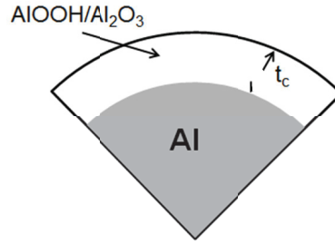
Figure 14: Schematic description of aluminum particle and a penetration thickness t_c . The unreacted aluminum core results in a hydrogen yield of less than 100%.
