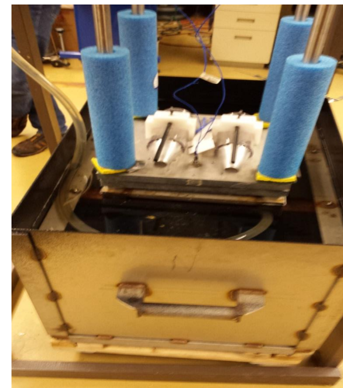
Figure. 1: Blast device
