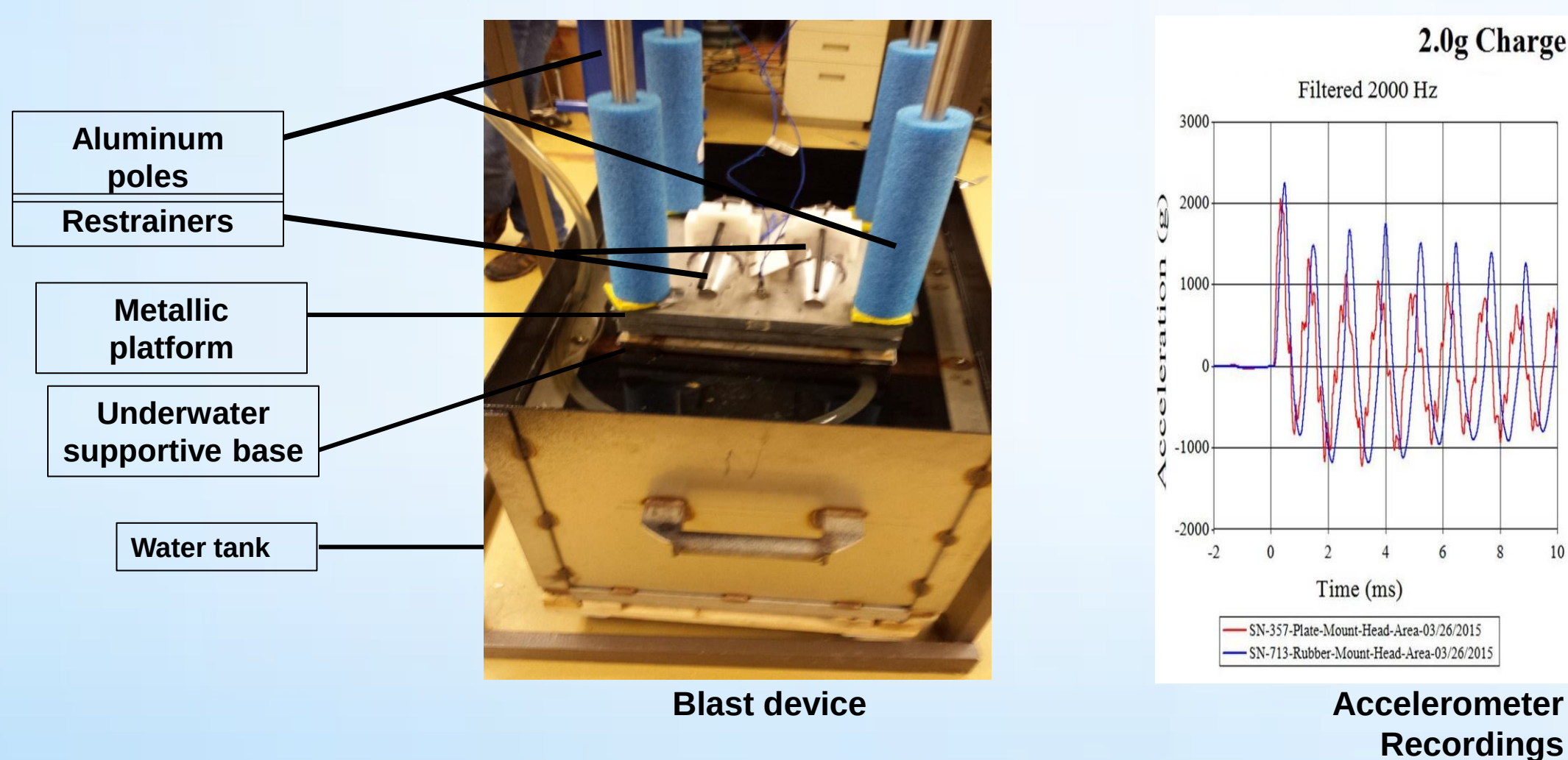
Figure 1. Underbody blast device with sample accelerometer recordings
