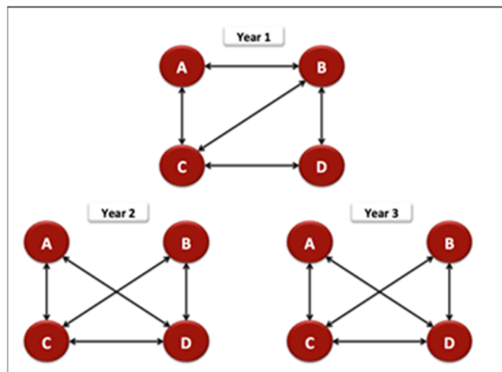
Figure 1. Critical Node Analysis for a Synthetic Network
