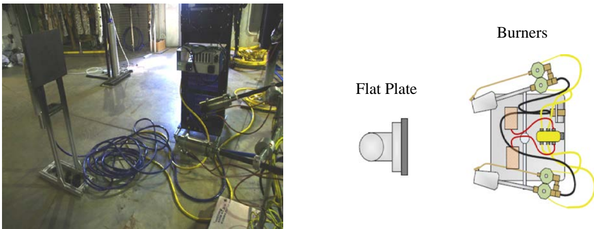
Figure 7. Flat plate test form with two burners/one stand
