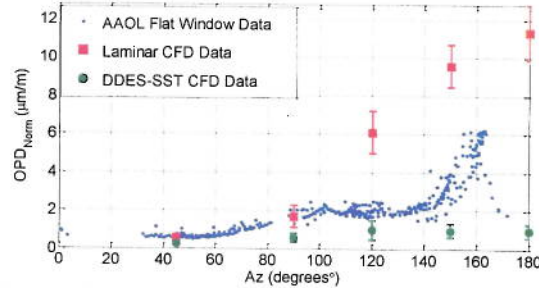
Figure 5. AAOL experimental data compared with CFD data. 3
