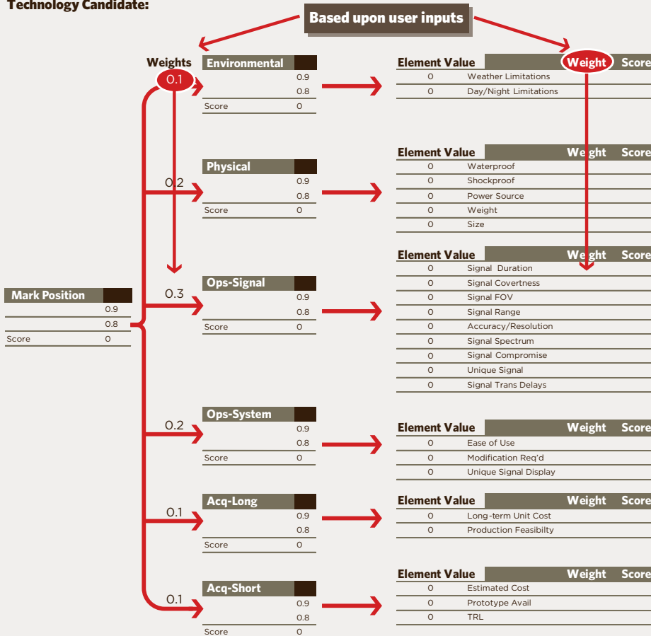
FIGURE 3. SAMPLE OBJECTIVES HIERARCHY
