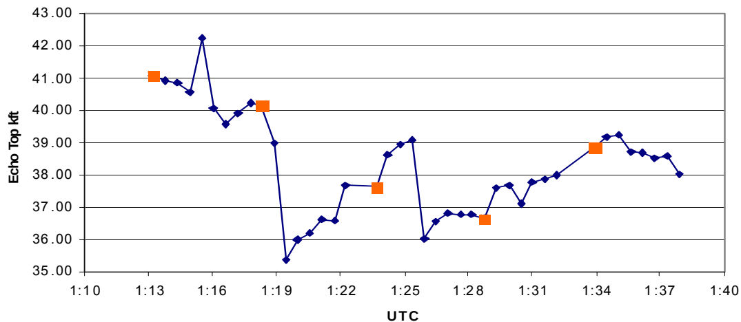
Figure 10: Echo top height vs. time for the storm cell depicted in Figure 9 with time resolution of 34 s (blue diamonds) and 5 minutes (orange squares)
