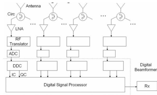
Figure 7: MPAR Implementation Using a Digital Beamformer
