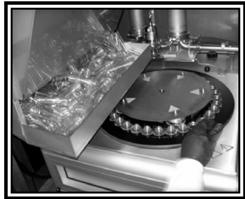
Blow Mold Heating Carrousel
