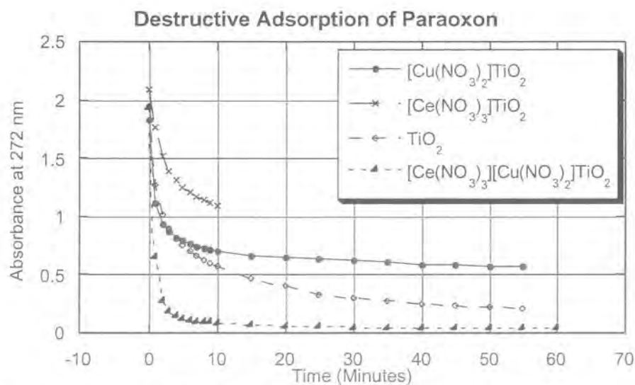
Figure 20. Destructive Adsorption of Paraoxon by Various TiO 2 Samples.
