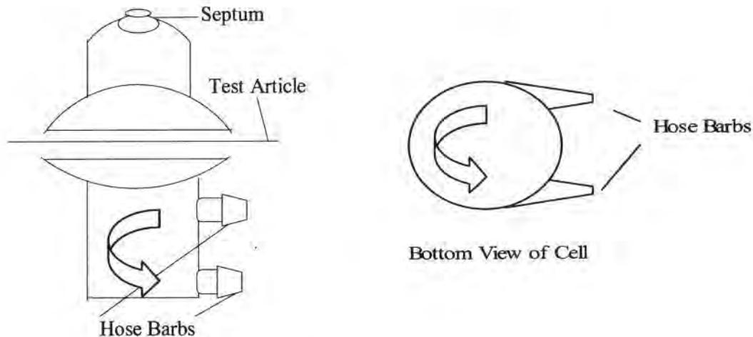
Figure 1. Permeation Cell
