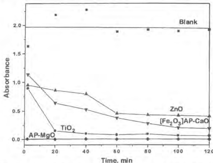
Figure 6: Rate of disappearance of paraoxon (4.5- \mu L) on various metal oxide samples (0.1-g). Lower intensity indicates more destructive adsorption of paraoxon.
