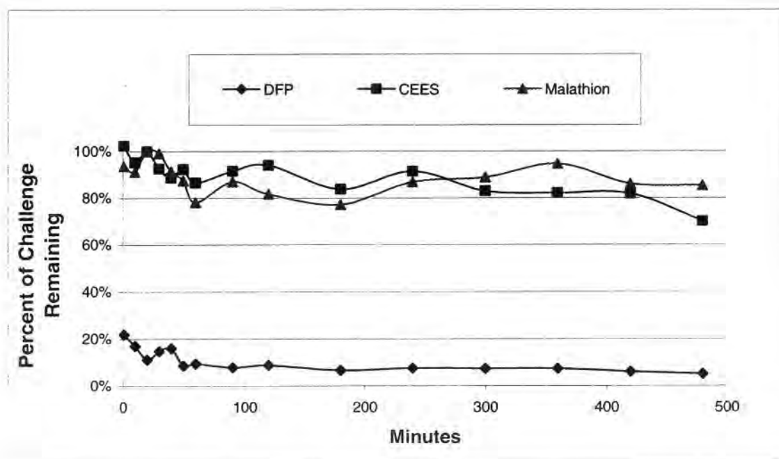
Figure 15. Simulant Depletion with Time Using La(Krytox®) 2
