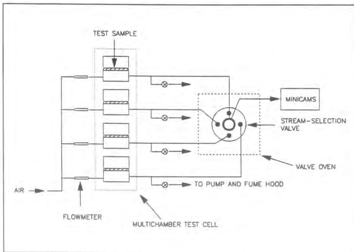
Figure 1 Schematic diagram of the permeation test system.
