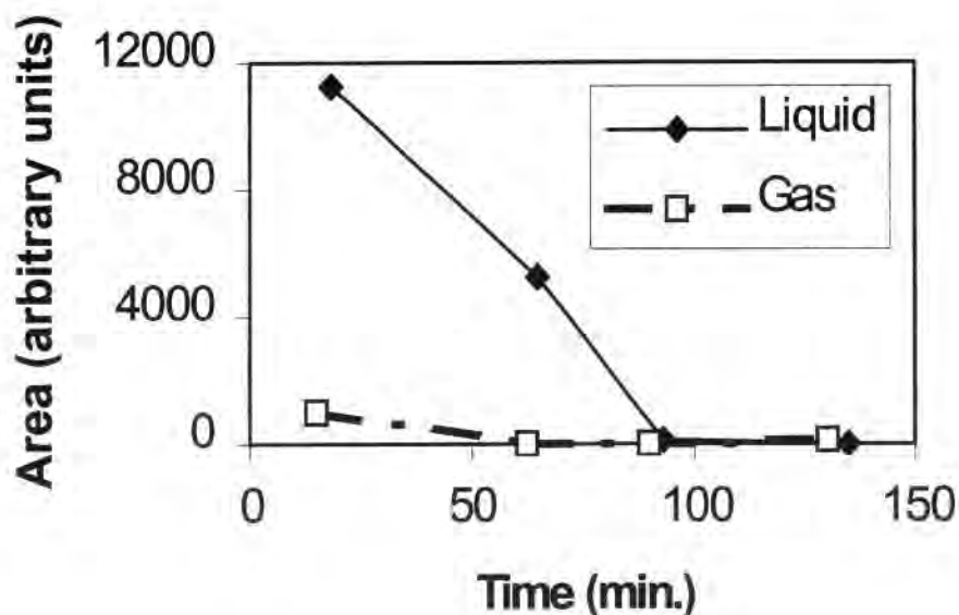
Figure 3. Plot of area of dimethyl sulfide GC peak versus time using a 3% H_2O_2 oxidant and a H_5PV_2Mo_{10}O_{40} catalyst.
