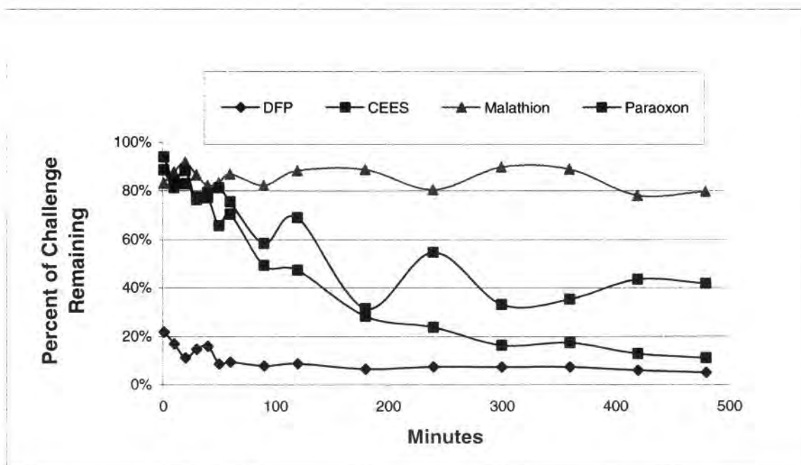
Figure 12. Simulant Depletion with Time Using Cu(Krytox®)₂
