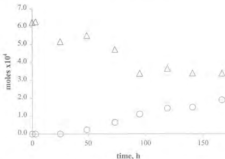
Figure 38. The heterogeneous, ambient-temperature air oxidation of (CH 3 CH 2 SCH 2 CH 2 Cl, CEES; \Delta ) to (CH 3 CH 2 S(O)CH 2 CH 2 Cl, CEESO; \circ ) catalyzed by Ag 5 1 powder under ambient conditions (room temperature and 1.0 atm air). CEES (0.275 M) and Ag 5 1 in 2,2,2-trifluoroethanol with 1,3-dichlorobenzene (internal standard) were stirred at 400 rpm in 18-mL glass vials fitted with Teflon septa. CEES and CEESO were quantified by GC.
