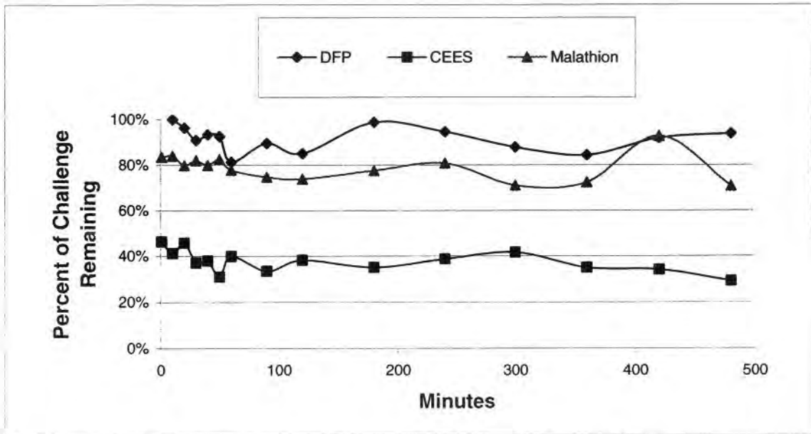
Figure 16. Simulant Depletion with Time Using Perfluoropropionic Acid
