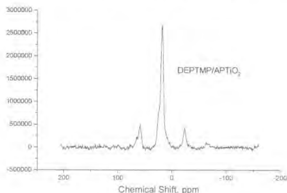
Figure 51. 31 P NMR Spectrum of DEPTMP/APTiO 2
