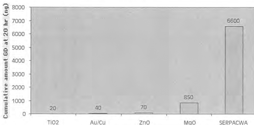
Figure 48. Cumulative amount GD vapor permeating through the aTSP after 20 hr as measured by penetration cell model / MINICAMs systems (saturated GD vapor, 0.15 mm thickness).
