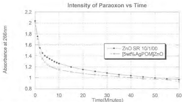
Figure 11. Destructive Adsorption of Paraoxon with Coated and Uncoated ZnO
