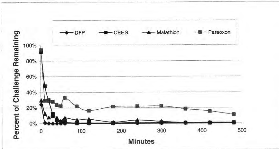
Figure 19. Simulant Depletion with Time Using METSS 2-8-14
