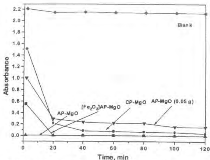
Figure 4: Rate of disappearance of paraoxon (4.5-µL) on magnesium oxide samples. Lower intensity indicates more destructive adsorption of paraoxon.
