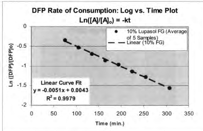
Figure 10 – Plot of \text{Ln}([\text{DFP}]/[\text{DFP}]_0) vs. time for the average of five Incroquat/10% by wt. Lupasol FG samples. The dotted black dotted line is a linear curve fit.
