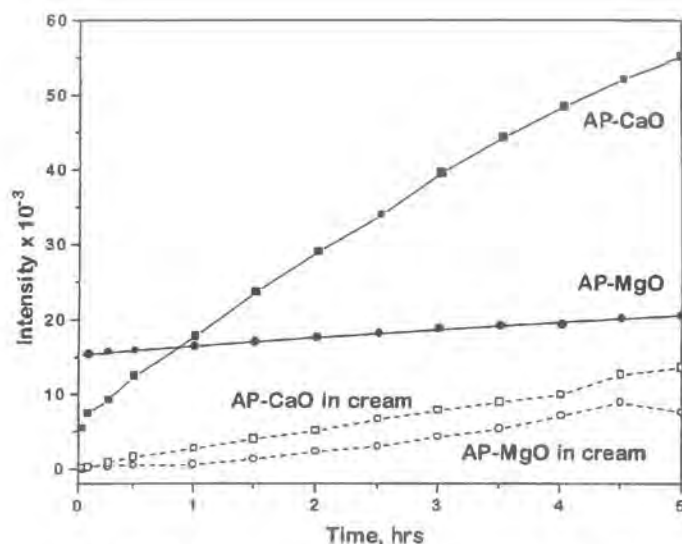
Figure 14: Appearance of ethyl vinyl sulfide during reaction of 2-CEES on metal oxides with and without the base cream. Higher intensity indicates more destructive adsorption of 2-CEES.
