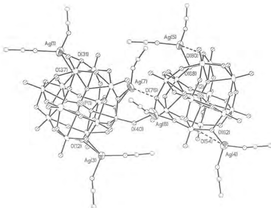
Figure 37. Structure of Ag 51 crystallized from MeCN and Et 2 O (formula: Ag 10.4 P 2 V 4 Mo 20 O 80 (NO 3 ) 0.4 •(MeCN) 17.3 (H 2 O) 1.5 ). Each metal position on the POM has 1/6 V character and ca. 5/6 Mo character. Selected average bond lengths (Å) and angles (deg): Ag - O t , 2.40; Ag - O b , 2.49; Ag - N s , 2.24; P - O c , 1.53; Mo - O t , 1.68; Mo - O b , 1.96; O c - Mo, 2.42; O b - Ag - O b , 62.9; Mo - O b - Mo, 89.0; O c - P - O c , 109.4; where O t = terminal oxygen, O b = μ 2 -oxo, O c = μ 3 -oxo, N s = acetonitrile (solvent) nitrogen. Solvent (MeCN and H 2 O) and silver ions not bound to the POM units have been omitted for clarity.
