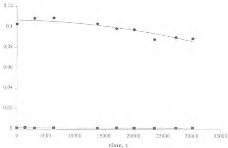
Figure 40. Adsorption of CEES onto the solid catalyst Ag 5 1. Concentrations of CEES (●) and the hydrolysis product (CH 3 CH 2 SCH 2 CH 2 OH (■)) are plotted versus time. After 8.4 hours, 5.26 x 10 -5 mols of CEES was absorbed onto 3.53 x 10 -5 mols of catalyst. No CEESO was detected.
