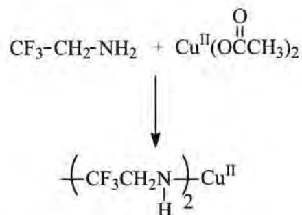
Figure 2 Synthesis of fluorocarbon-functional-amine-copper catalysts
