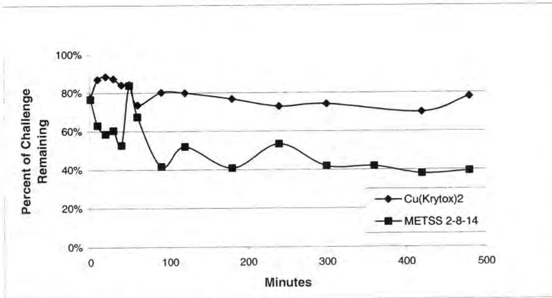
Figure 28. Depletion of DEET in Cu(Krytox®) 2 and METSS 2-8-14
