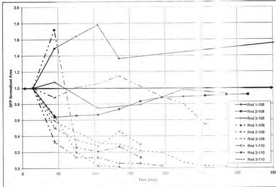
Figure 17: Relative amount of DFP in headspace of designated samples vs. time, as measured by HS-SPME and GC-MS. TNSP 3 (dotted line), TNSP 4 (dotted/dashed line) and TNSP 3/4 Control (solid line). Formulations are Water-in-Oil, Hydrophobic Clay Dipropylene Glycol Dibenzoate Emollient.
