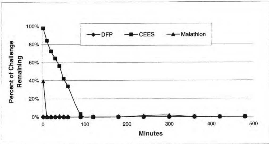
Figure 18. Simulant Depletion with Time Using METSS 2-8-13
