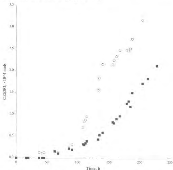
Figure 39. Reaction profile for the ambient-temperature air oxidation of CEES (O) to CEESO catalyzed by Ag 5 1 in 2,2,2-trifluoroethanol and its inhibition by added DMSO (■).
