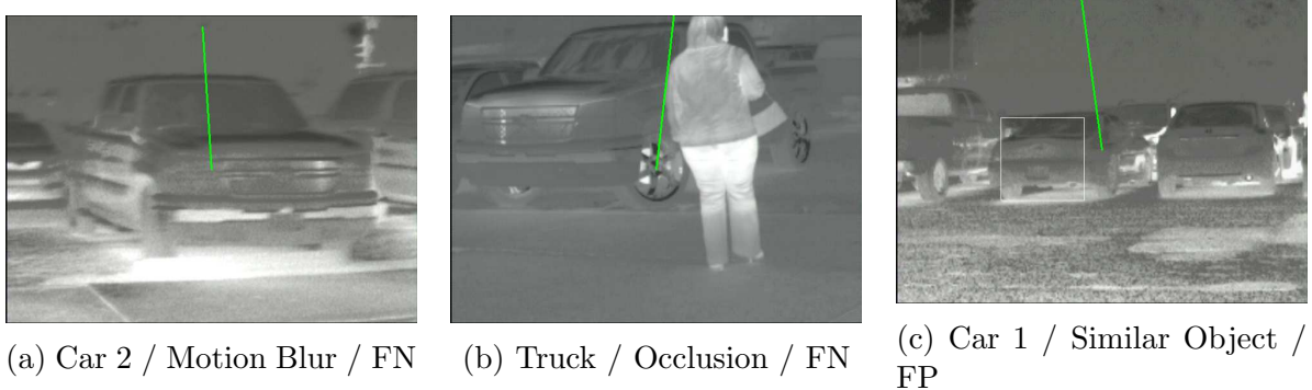
Figure 5.2: Examples of Tracking Error
