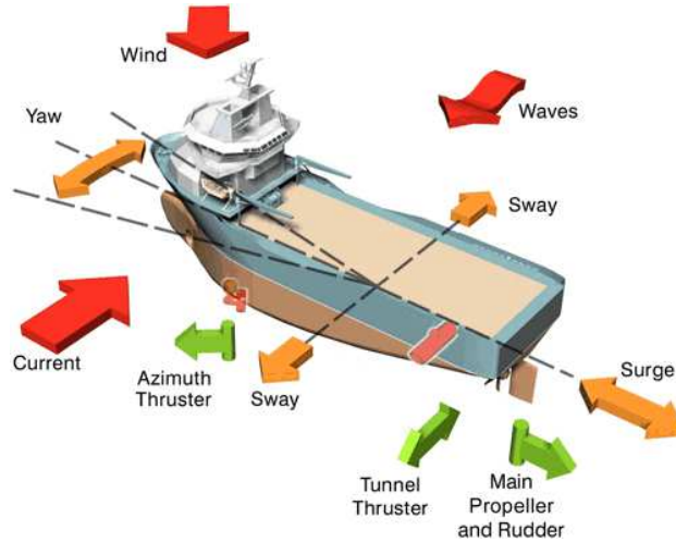
Figure 2.2: Forces acting on a marine vessel
