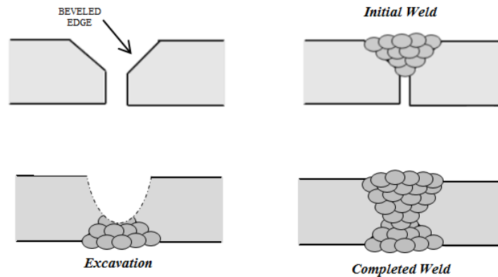
Figure 10. Generic Specimen Welding Sequence.
