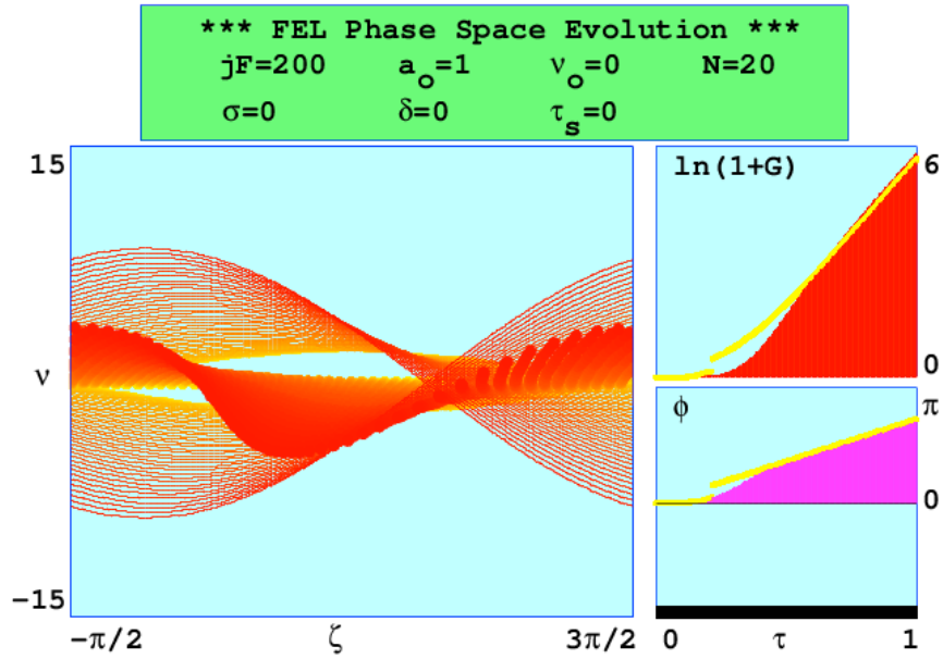
Figure 6. Phase space plot at high current density when j = 200 and \nu = 0 (i.e., at resonance)
