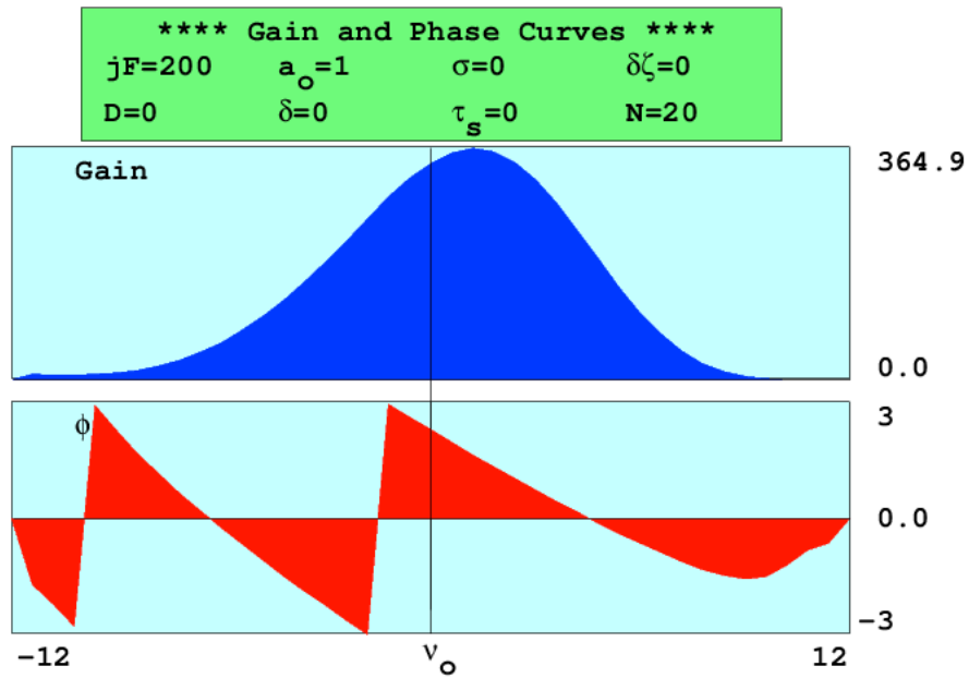
Figure 7. Gain and phase spectrum plot at high current density when j = 200 and \nu = 0 (i.e., at resonance)
