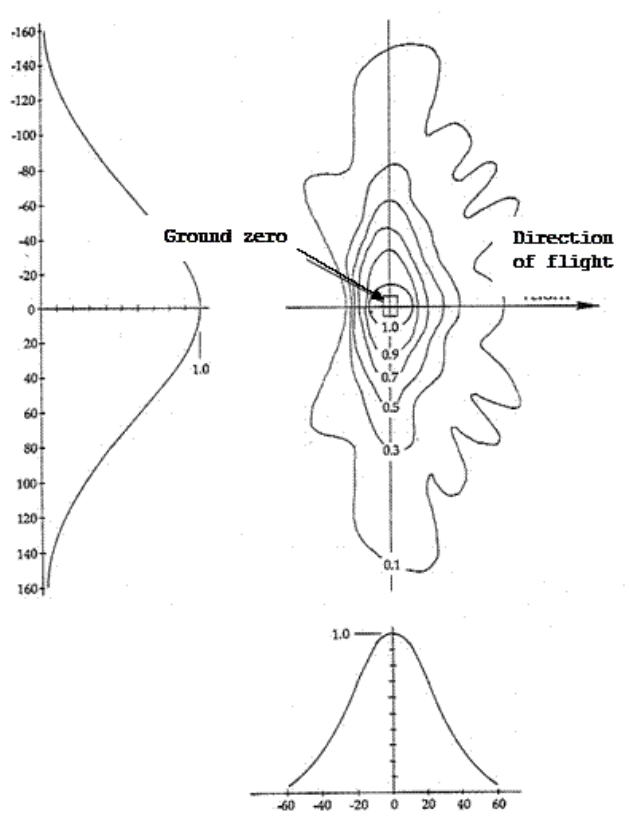
Figure 20. PD contour lines of LAM damage matrix, from [4]
