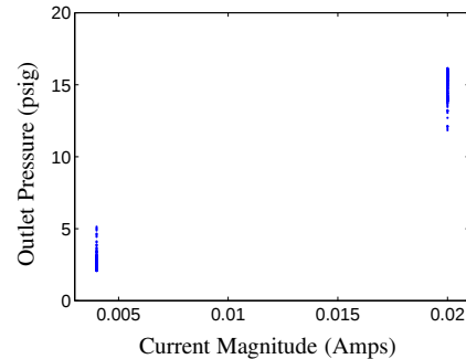
Figure 12. Current magnitude vs. output pressure
