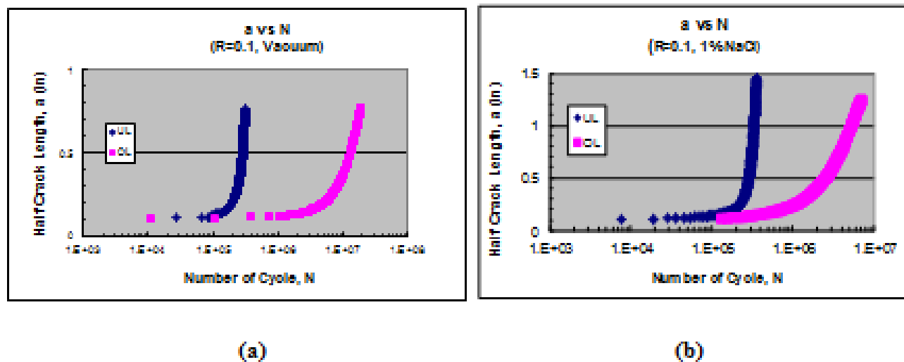
Figure A-5: Variation of Half Crack Length with Number of Loading Cycle at R=0.1 in a Vacuum and 1 Percent NaCl Solution under Overloading and Underloading
