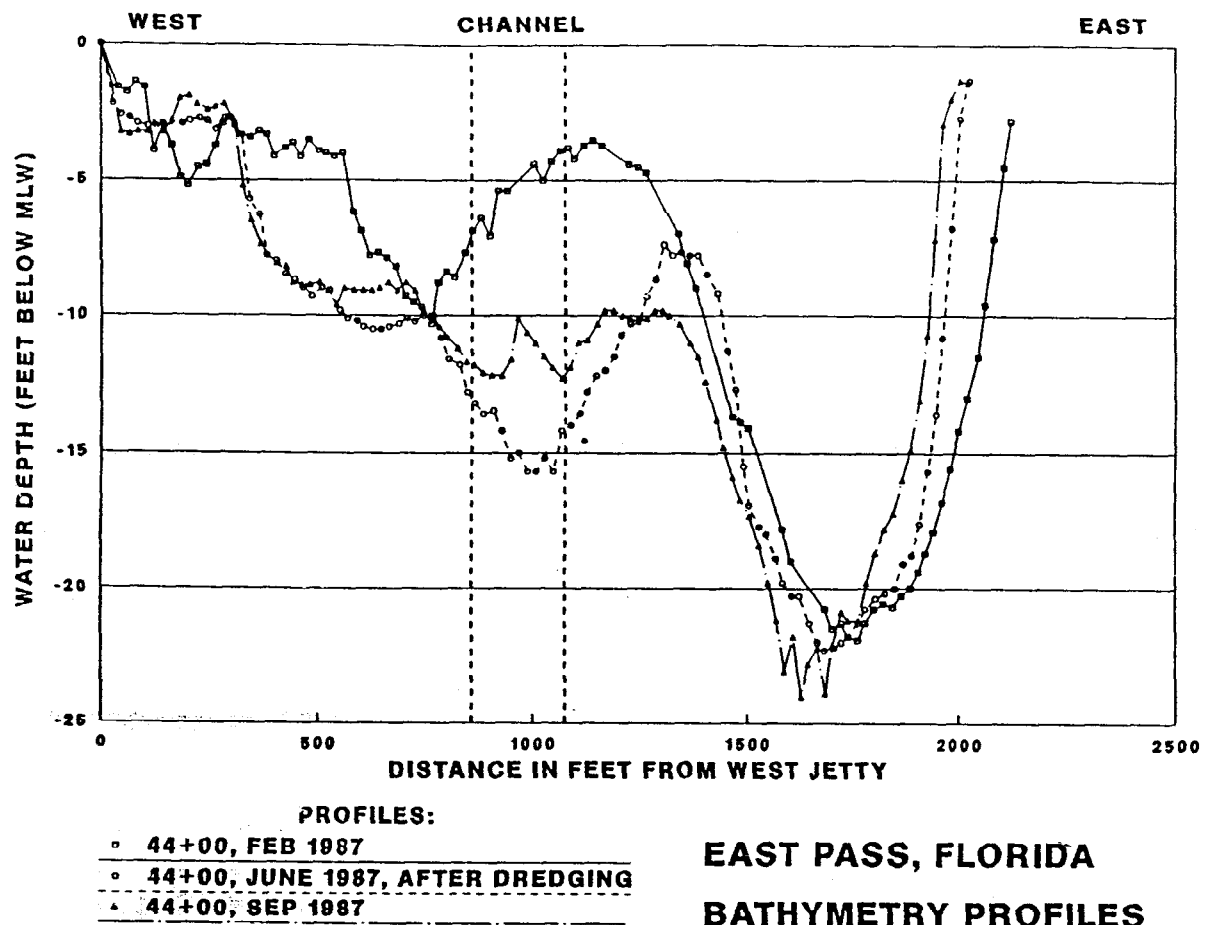
Figure 4. Profiles along line 44+00
