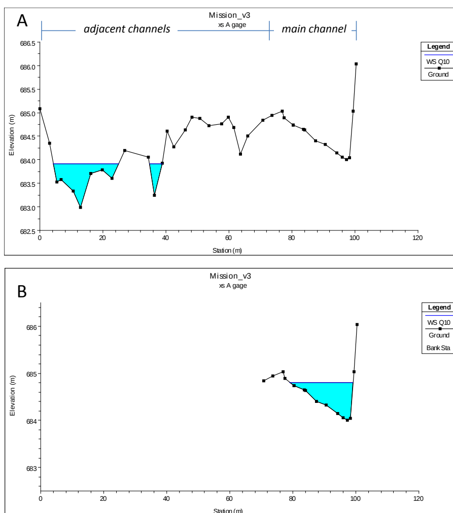
Figure 9. The effect of multiple channels on the simulated water surface of a 10-year recurrence-interval flow at Mission Creek near Desert Hot Springs, CA. Panel A shows the entire valley width with flows erroneously modeled in disconnected areas. Panel B shows only areas connected to upstream areas and more accurately simulates the flow location, depth, and width.
