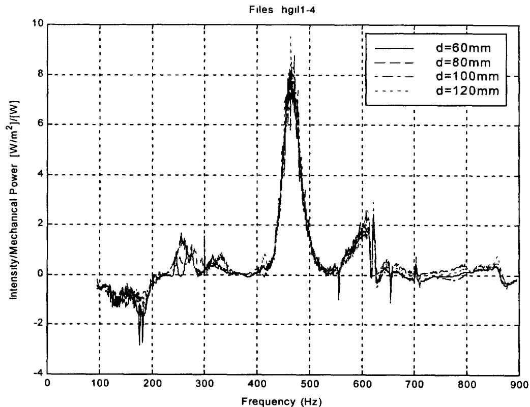
Figure 5.6: Measured intensity spectra for 4 hydrophone spacings.
