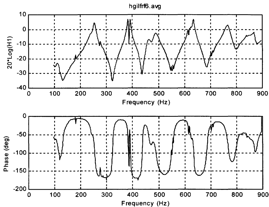
Figure 5.8: Measured FRF of 9.5mm thick bare plate.
