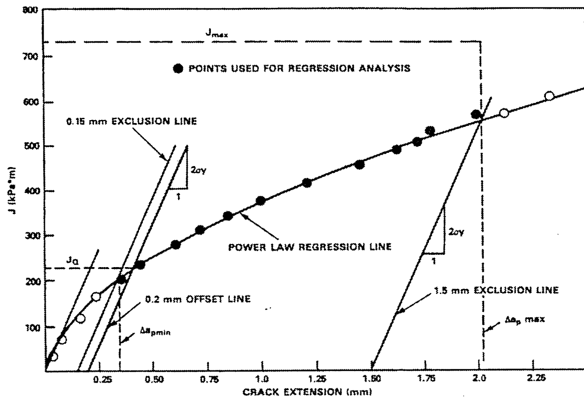
FIGURE 2.: A typical J-crack growth resistance curve [1].
