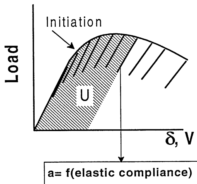
FIGURE 3.: Unloading compliance method load-displacement record.
