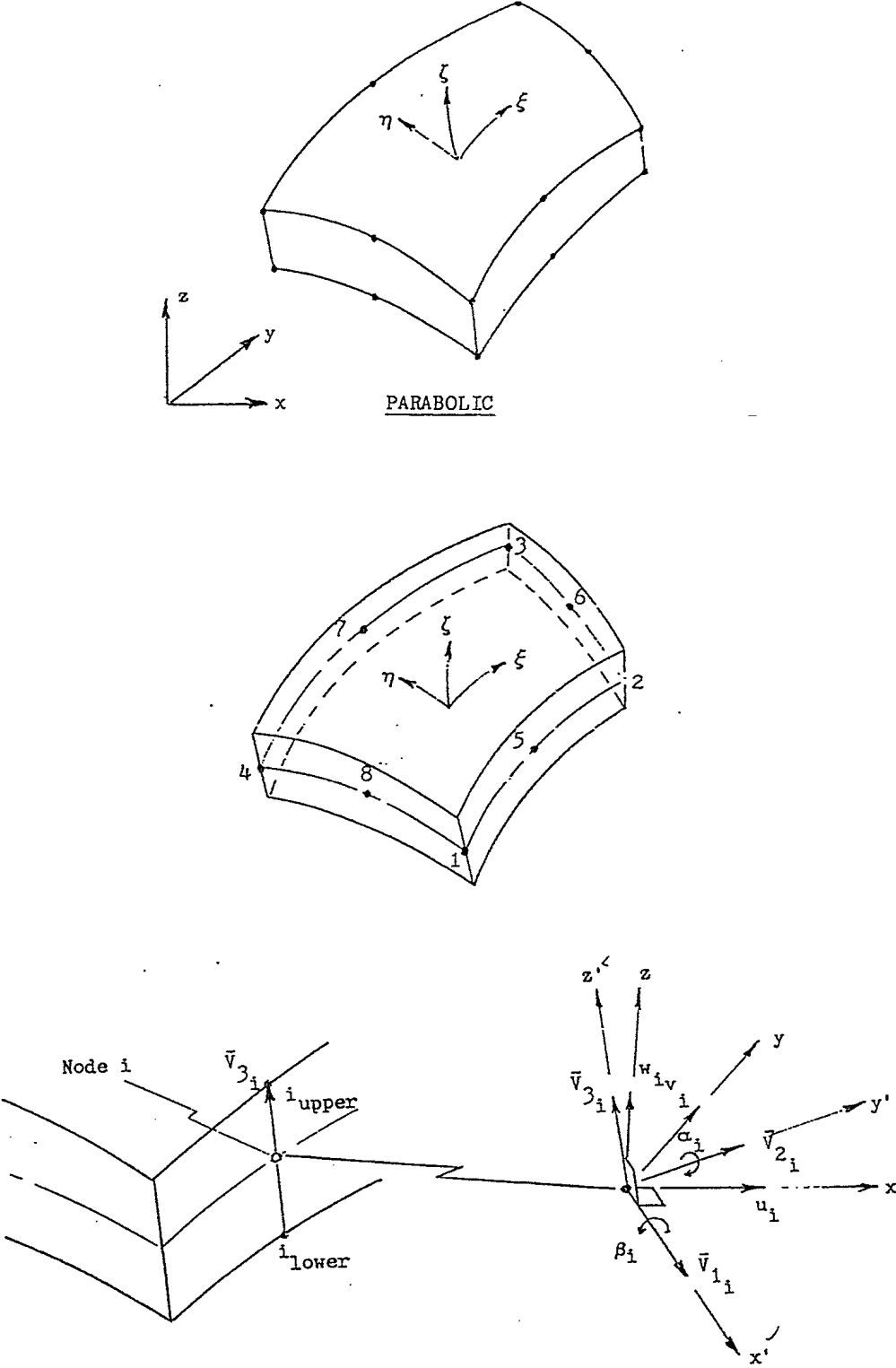
FIGURE 8.1: Curved Shell Elements
