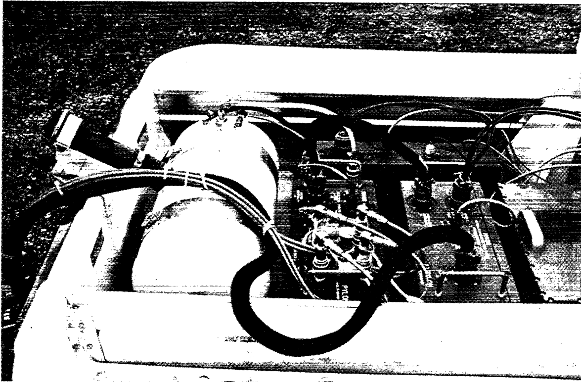
Figure 2. Remote vehicle electronics compartment
