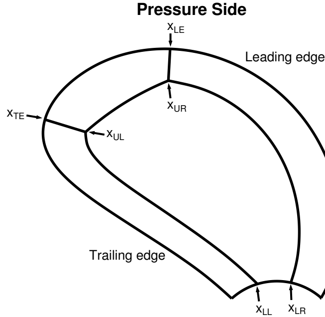
Figure 3: The points used to split the blade into separate surfaces.
