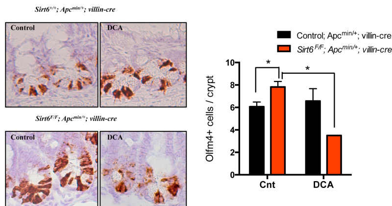
Figure 1. Expansion of ISCs in Sirt6 fl/fl ; Villin-cre; Apc min mice. Representative pictures of Olm4 in situ hybridization showing ISC staining (left panels) and quantification of Olm4 positive cells (right panel) in the intestines of control and Sirt6 fl/fl ; Villin-cre; Apc min mice treated or untreated with DCA.
