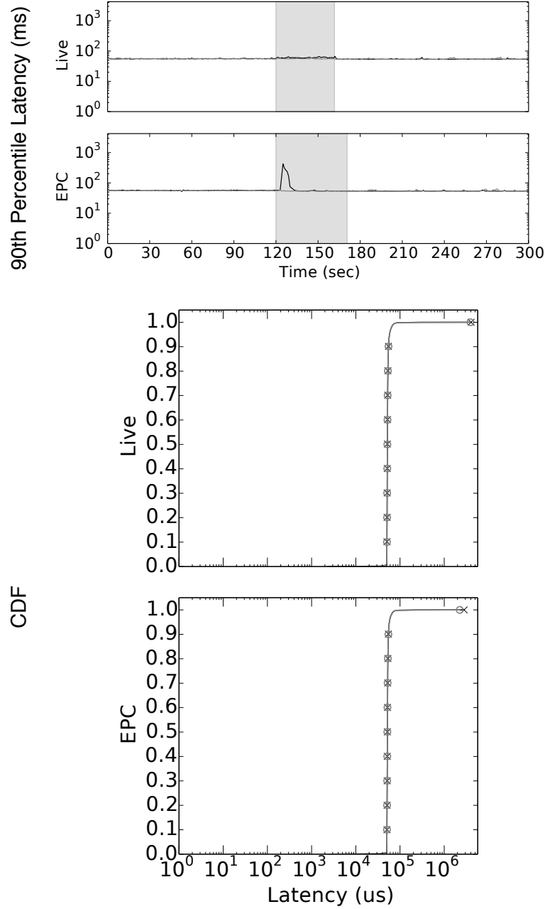
Figure 13: Latency with MySQL at 10 Gbps. The black and gray lines correspond to the migrated and contending VMs, respectively. The top two graphs show the 90th percentile latency over time on a log scale, with the shaded areas indicating the duration of migration. The bottom two figures are CDFs of the response latencies during the 5-minute period, with markers at every 10th percentile.
