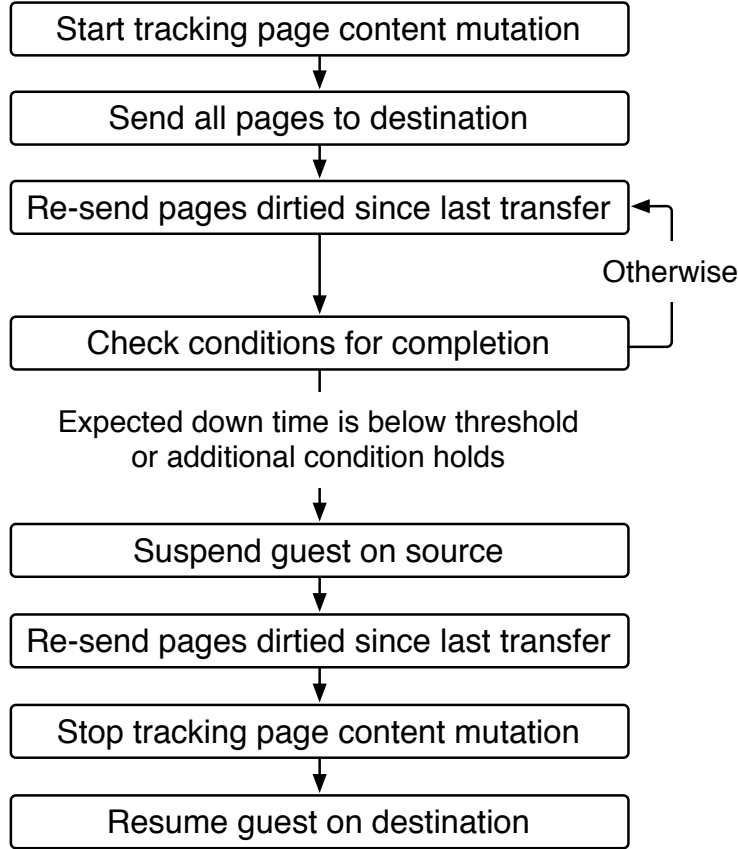
Figure 4: Live Migration Algorithm
