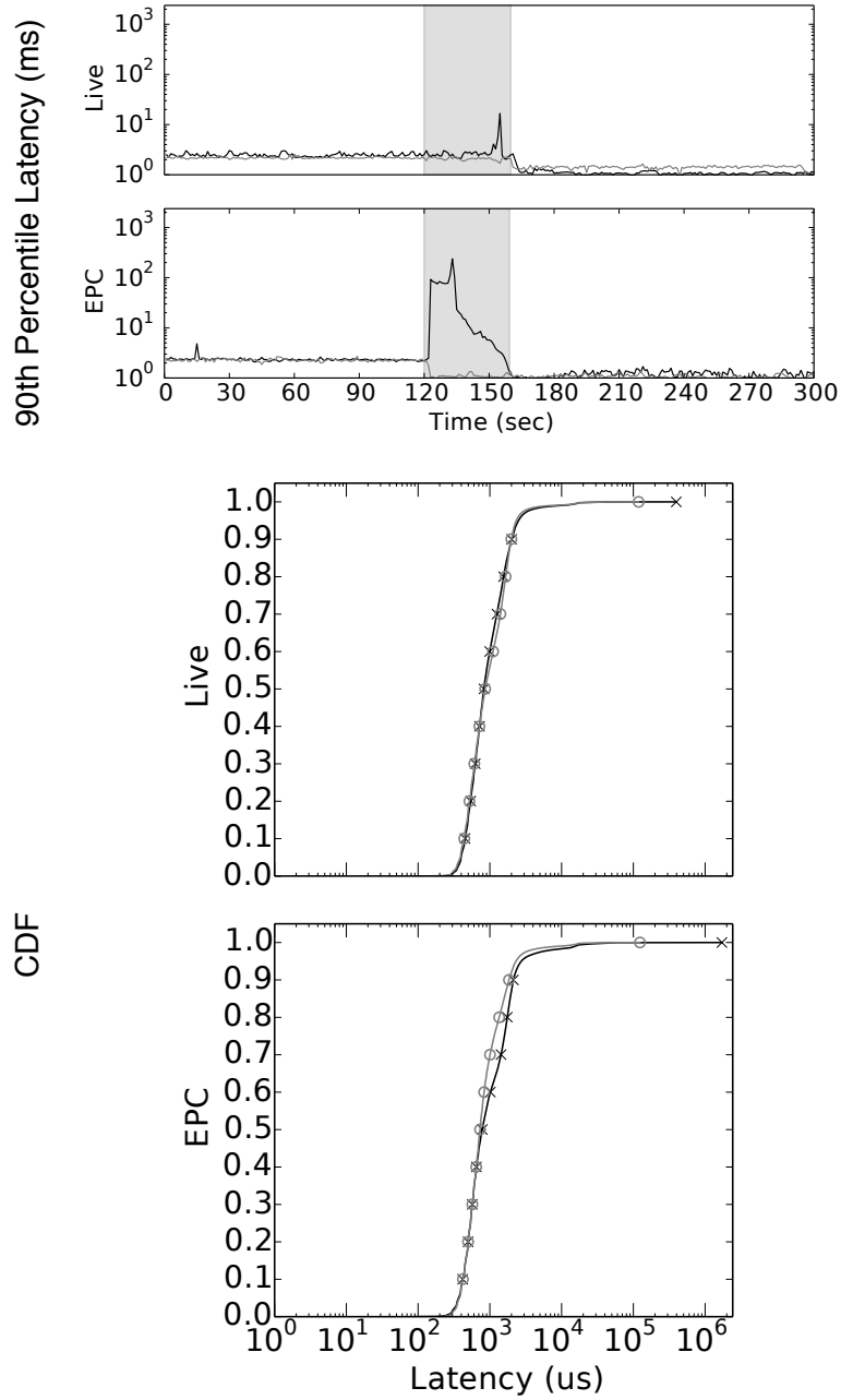
Figure 11: Latency with Memcached at 10 Gbps. The black and gray lines correspond to the migrated and contending VMs, respectively. The top two graphs show the 90th percentile latency over time on a log scale, with the shaded areas indicating the duration of migration. The bottom two figures are CDFs of the response latencies during the 5-minute period, with markers at every 10th percentile.
