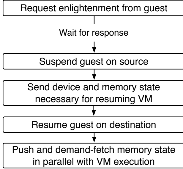
Figure 7: Workflow of Enlightened Post-Copy Migration
