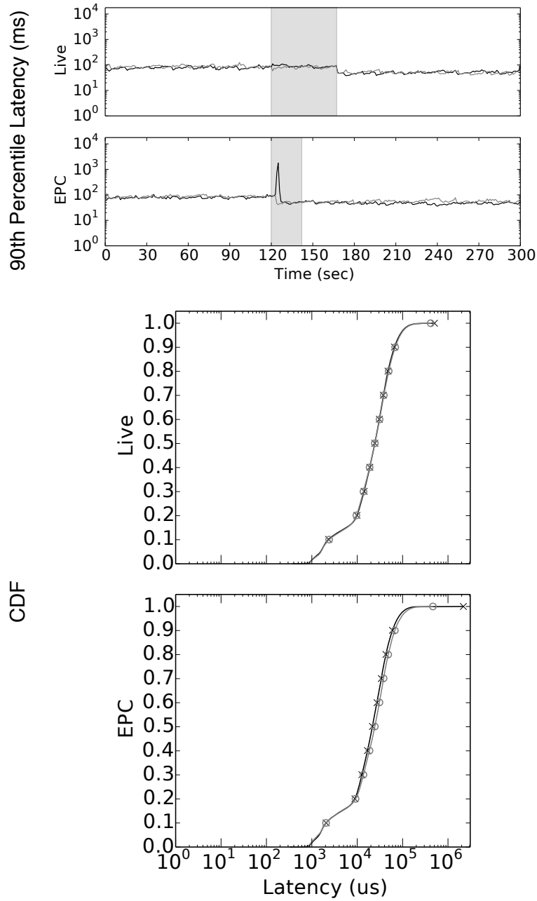
Figure 15: Latency with Cassandra at 10 Gbps. The black and gray lines correspond to the migrated and contending VMs, respectively. The top two graphs show the 90th percentile latency over time on a log scale, with the shaded areas indicating the duration of migration. The bottom two figures are CDFs of the response latencies during the 5-minute period, with markers at every 10th percentile.
