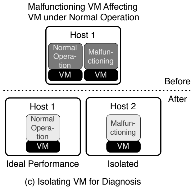
Figure 1: Scenarios for Urgent VM Eviction
