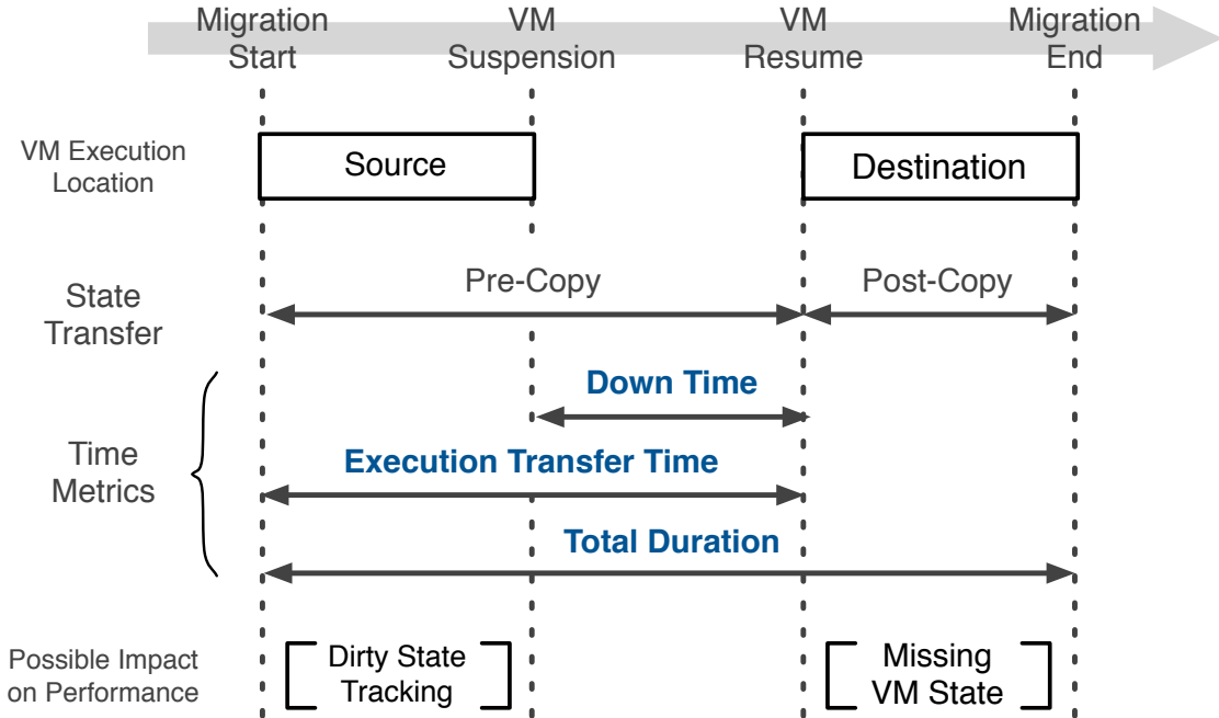
Figure 3: Overview of Migration Mechanics
