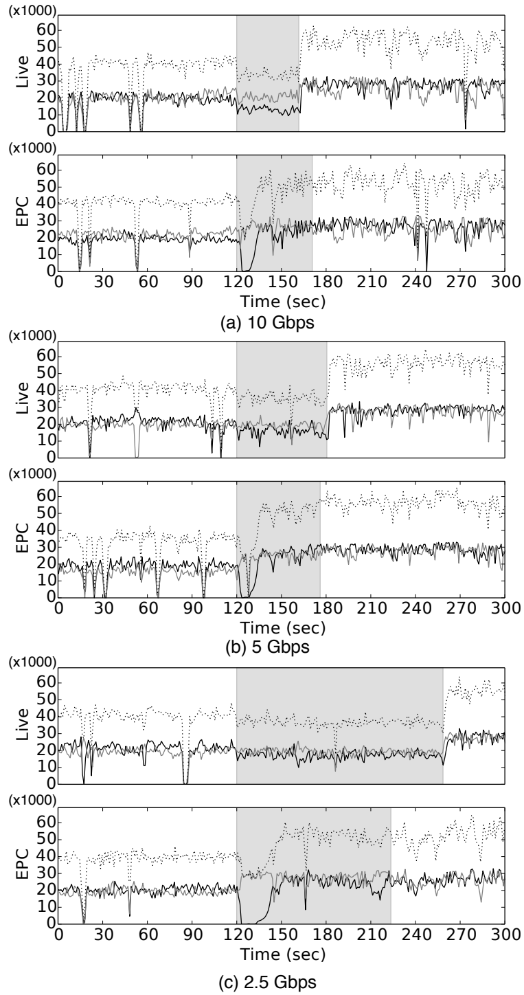
Figure 12: End-to-End Results with MySQL. The y-axis indicates throughput in operations or transactions per second. The black and gray lines represent the migrated and contending VMs, respectively, and the dotted lines the aggregate of the two. The shaded areas show the duration of migration.
