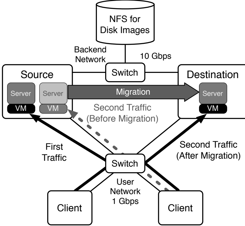
Figure 9: Experiment Set-Up
