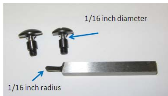
Figure 10. Sample preparation for the screw tensile strength tests. A rounded lathe tool bit is used to reduce the diameter of a region of the screw shoulders to about 1/16 inch.
