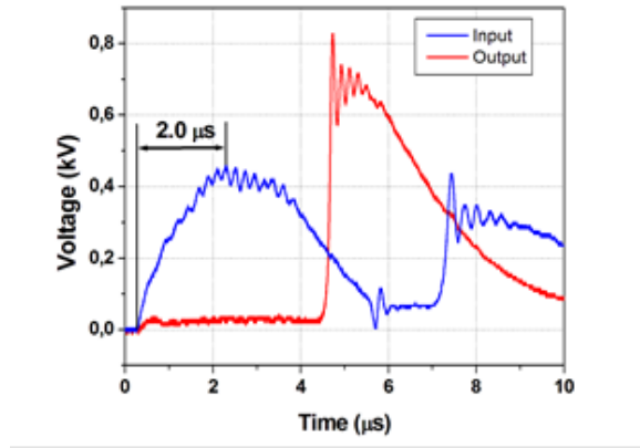
Fig. 22. RF soliton generation at line output using capacitor C#2.
