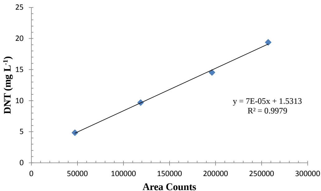
Figure B 11. GC-MS calibration curve 5 – 20 \text{mg L}^{-1} DNT for GAC kinetic experiment
