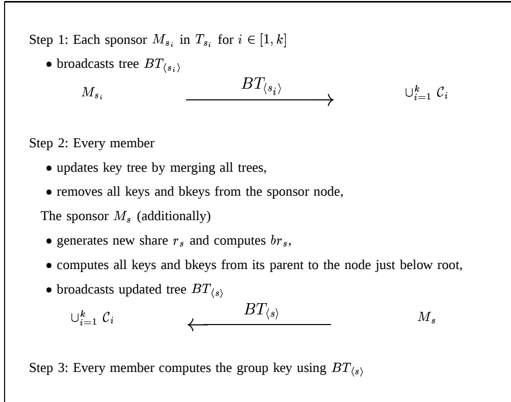
Fig. 7. MERGE Protocol
