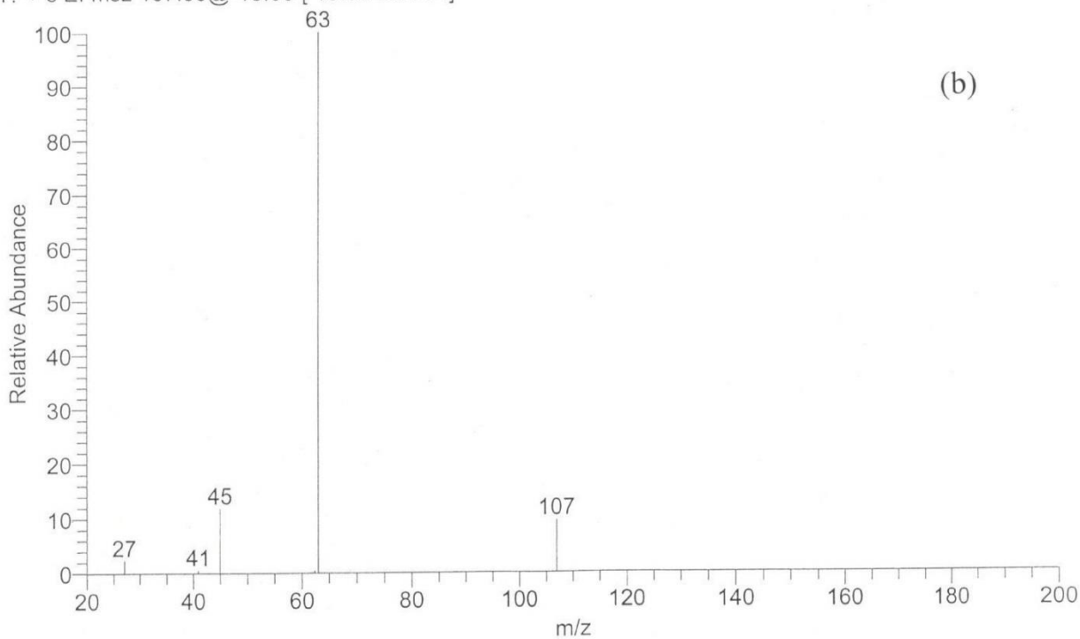
Figure 9. Mass spectra for compound 8 : (a) EI and (b) CID at m/z 107.
