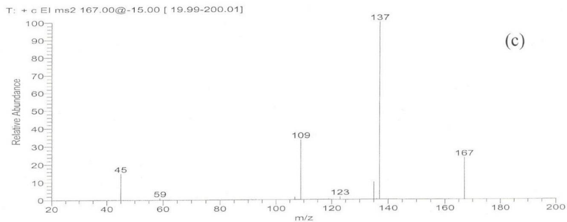
Figure 4. Mass spectrum for compound 3: (a) EI, (b) CID at m/z 137, and (c) CID at m/z 167.
