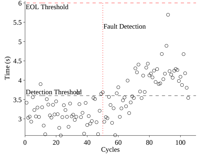
Figure 10. Valve close times with a atmosphere leak.
