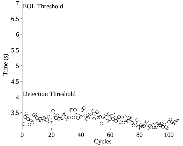
Figure 9. Valve open times with a atmosphere leak.
