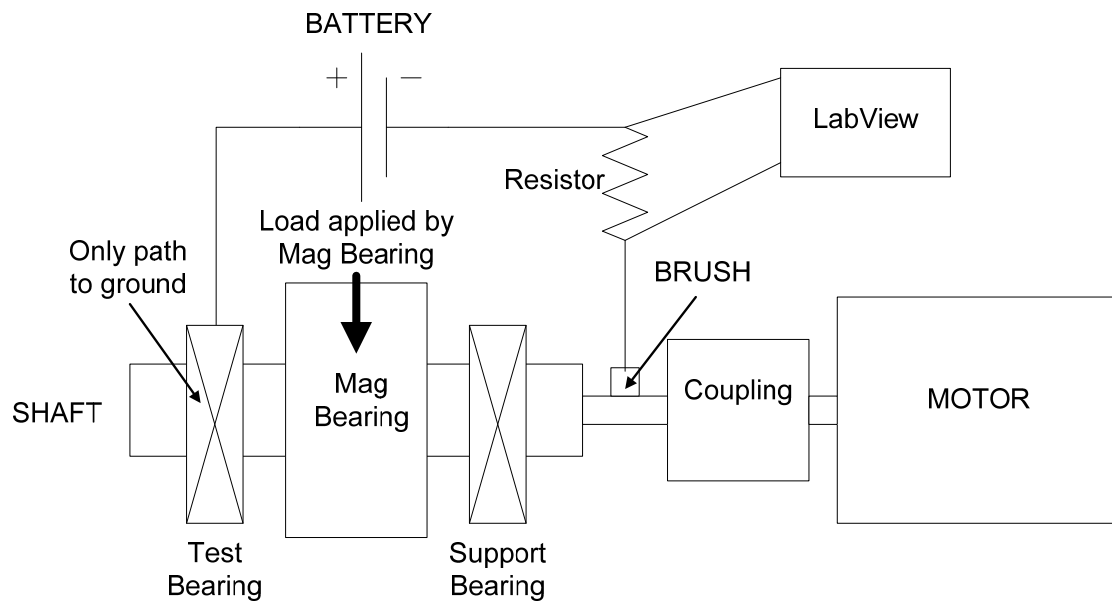
Fig. 22 Shaft circuit schematic showing load and ground
